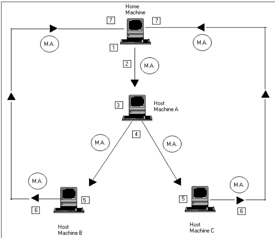
Figure 1. The life cycle of a mobile agent.
