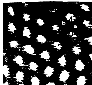
Figure 4. Atomic force microscopic image of an alkanethiol self assembled monolayer prepared on gold. The image has white and dark regions. White represents higher regions and dark represents lower regions at the surface. The distances between the white regions indicate that the image does not correspond to a clean gold surface. a and b correspond to nearest and next nearest neighbours, respectively. The micrograph is adapted from C A Alves, E L Smith and M D Porter, J. Am. Chem. Soc. , 114, 1222, 1992.
