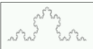
Figure 6. Stage 5 of Koch curve.
