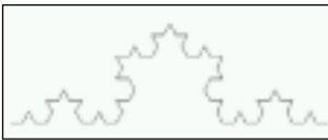
Figure 4. Stage 3 of Koch curve.
