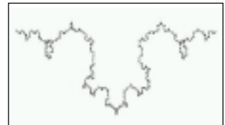
Figure 9. A random fractal.
