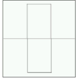
Figure 8. Generator of a fractal of integer dimension: the Peano curve.
