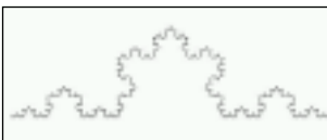
Figure 5. Stage 4 of Koch curve.
