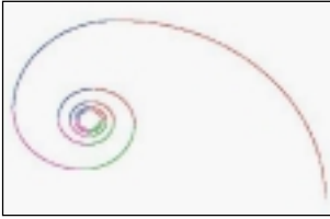
Figure 7. This curve is of infinite length and is in a bounded region but is not a fractal.
