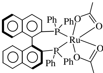
(S)-BINAP-Ru(OOCCH 3 ) 2
