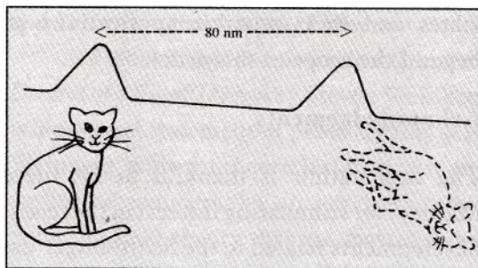
Figure 2. Wave packets entangled with the electronic states of the ion can be apart by as much as 80nm and thus have some quantum-classical features of the Schrodinger cat states.
