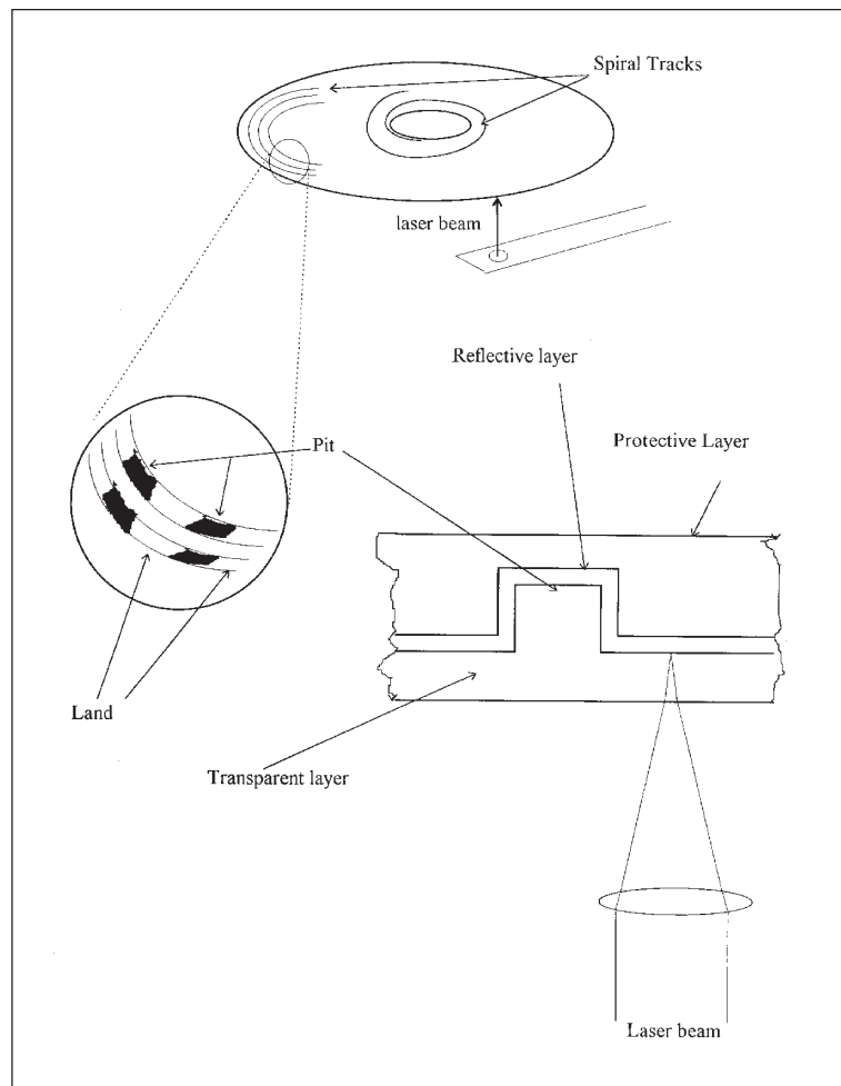
Figure 1 CD-ROM schematic.
