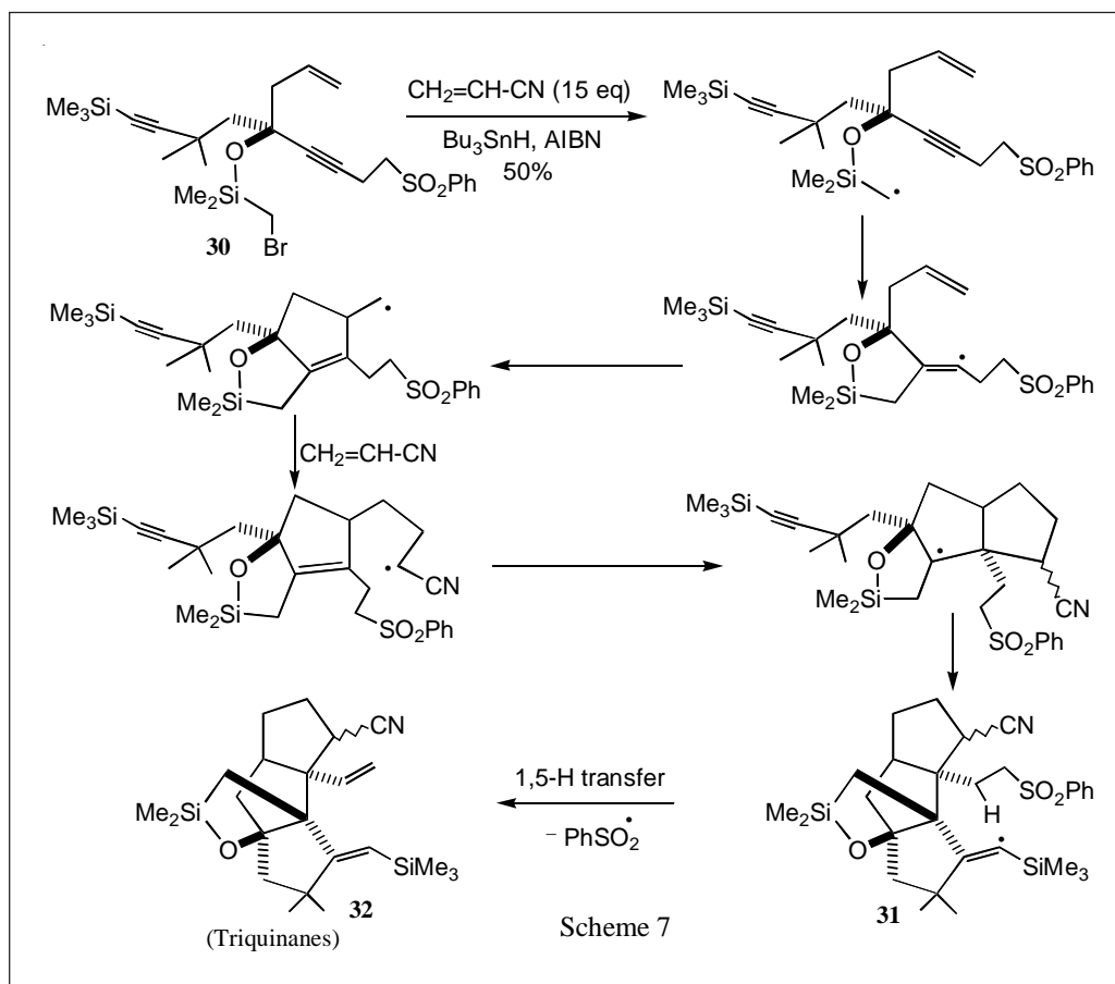
Scheme 7.
