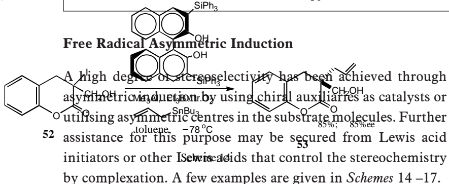
Schemes 12 and 13.
