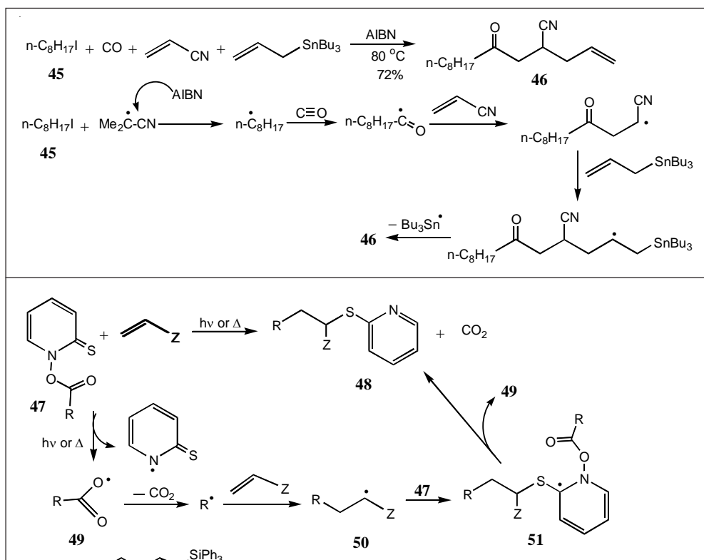
Schemes 12 and 13.
