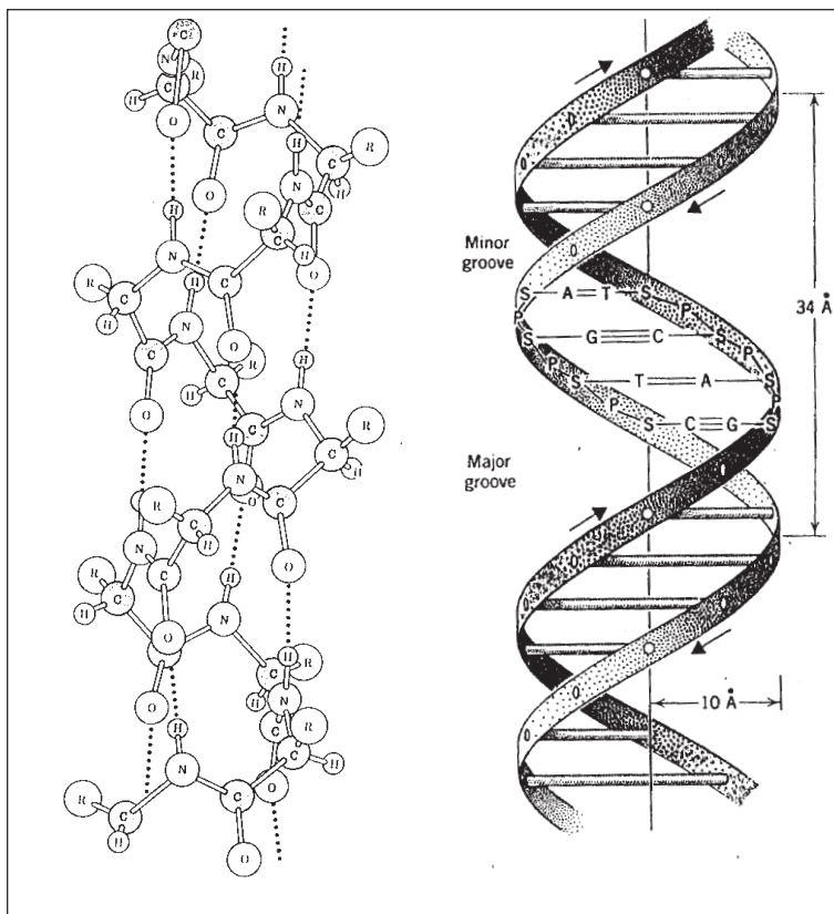
Figure 3 (left) An \alpha -helix. Note the N-H...O hydrogen bonds parallel to the helix axis.
