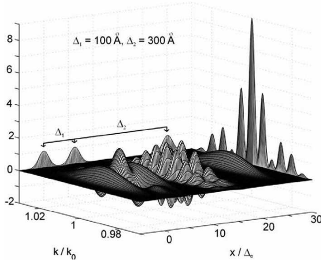
Figure 8. Triple humped Wigner function behind a double loop interferometer.
