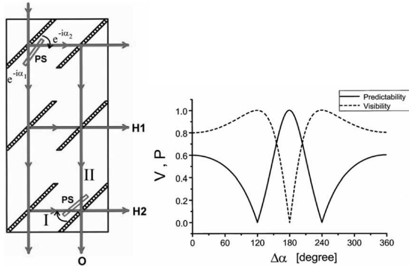
Figure 6. Double loop interferometer used to measure wave-particle properties and sketch of the experimental results [40].
