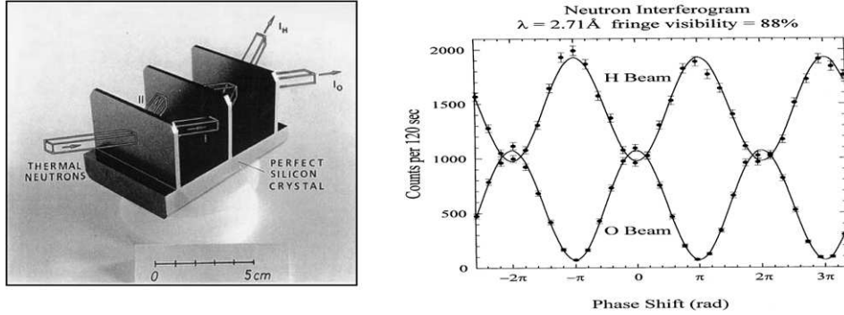
Figure 1. Sketch of a perfect crystal neutron interferometer and a typical interference pattern.
