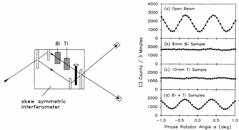
Figure 2. Phase-echo experiment using phase shifters with positive (Bi) and negative (Ti) coherent scattering lengths [25].
