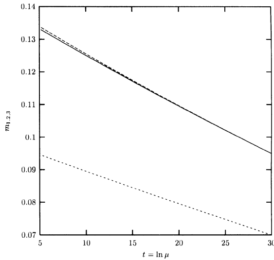
Figure 2. Evolution of the three neutrino mass eigenvalues in JM conjecture [11]. m_1 , m_2 and m_3 are represented by dashed line, solid line and dotted line respectively.
