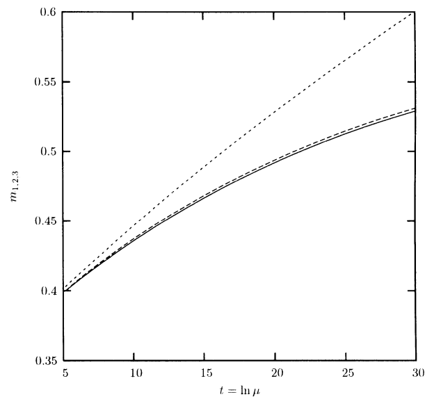
Figure 4. Evolution of the three nearly degenerate neutrino masses in MPR conjecture [12] (without the effect of scale-dependent VEV in II). m_3 , m_2 and m_1 are represented by solid line, dashed line and dotted line respectively.
