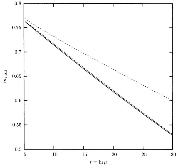
Figure 5. Evolution of the three nearly degenerate neutrino masses in MPR conjecture [12] (with the effect of scale-dependent VEV in I). m_3 , m_2 and m_1 are represented by solid line, dashed line and dotted line respectively.
