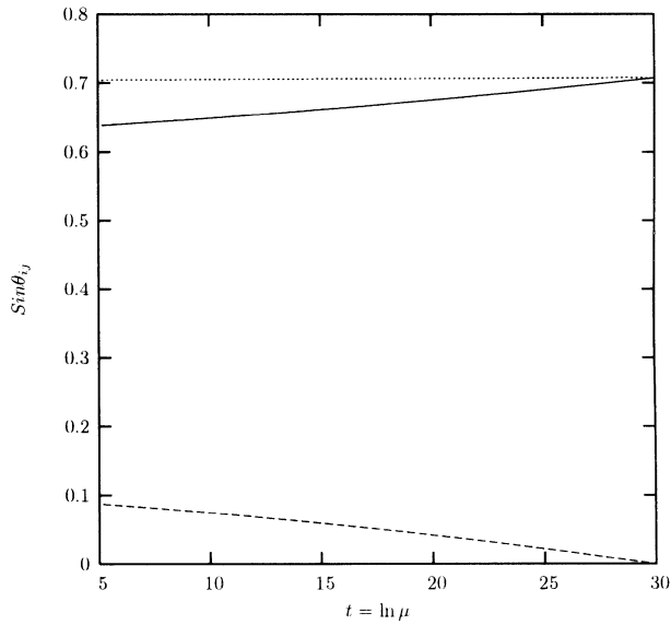
Figure 1. Evolution of the three mixing angles with energy scale in JM conjecture [11]. \sin \theta_{23} , \sin \theta_{13} and \sin \theta_{12} are represented by solid line, dashed line and dotted line respectively.
