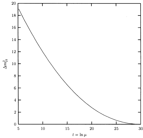
Figure 3. Evolution of the \Delta m_{21}^2 in JM conjecture [11] with energy scale. Its value at high-energy scale is zero.
