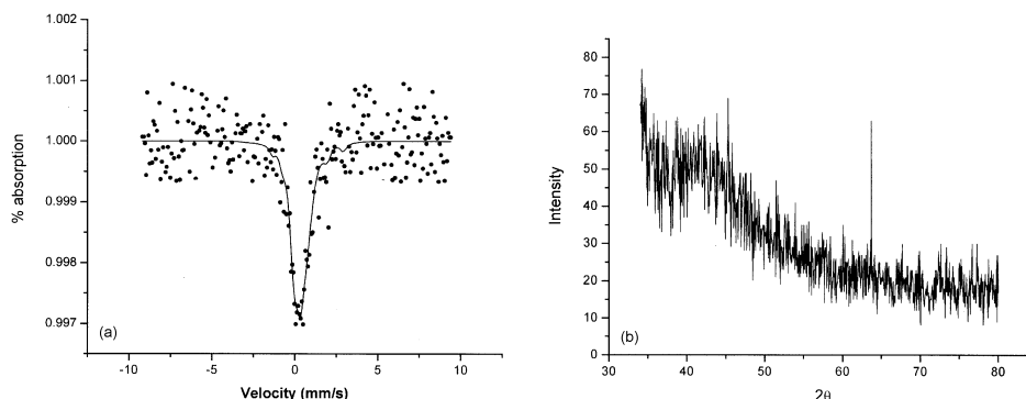
Figure 2. (a) The Mössbauer spectrum of the complex C_{42}H_{56}N_{12}Fe_2Cl_4O_8 at room temperature. The solid circles are experimental data points and the solid line is fitted to them. (b) X-ray diffraction pattern of the complex C_{42}H_{56}N_{12}Fe_2Cl_4O_8 .
