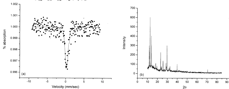
Figure 3. (a) The Mössbauer spectrum of the complex C_{18}H_{14}N_6FeCl_3O_6 at room temperature. The solid circles are experimental data points and the solid line is fitted to them. (b) X-ray diffraction pattern of the complex C_{18}H_{14}N_6FeCl_3O_6 .
