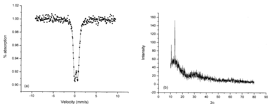
Figure 4. (a) The Mössbauer spectrum of the complex C_{11}H_{24}N_5S_2FeCl_2 at room temperature. The solid circles are experimental data points and the solid line is fitted to them. (b) X-ray diffraction pattern of the complex C_{11}H_{24}N_5S_2FeCl_2 .
