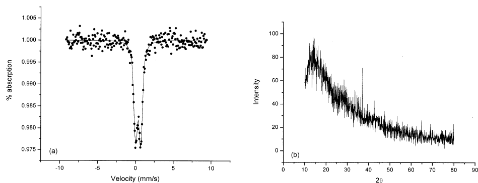
Figure 1. (a) The Mössbauer spectrum of the complex \text{C}_{48}\text{H}_{50}\text{N}_{10}\text{Fe}_2\text{Cl}_6\text{O}_8 at room temperature. The solid circles are experimental data points and the solid line is fitted to them. (b) X-ray diffraction pattern of the complex \text{C}_{48}\text{H}_{50}\text{N}_{10}\text{Fe}_2\text{Cl}_6\text{O}_8 .
