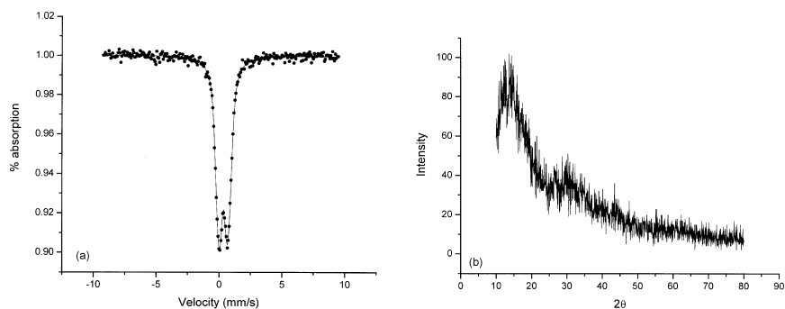
Figure 5. (a) The Mössbauer spectrum of the complex C_{11}H_{24}N_3S_2Fe(NO_3)_3 at room temperature. The solid circles are experimental data points and the solid line is fitted to them. (b) X-ray diffraction pattern of the complex C_{11}H_{24}N_3S_2Fe(NO_3)_3 .
