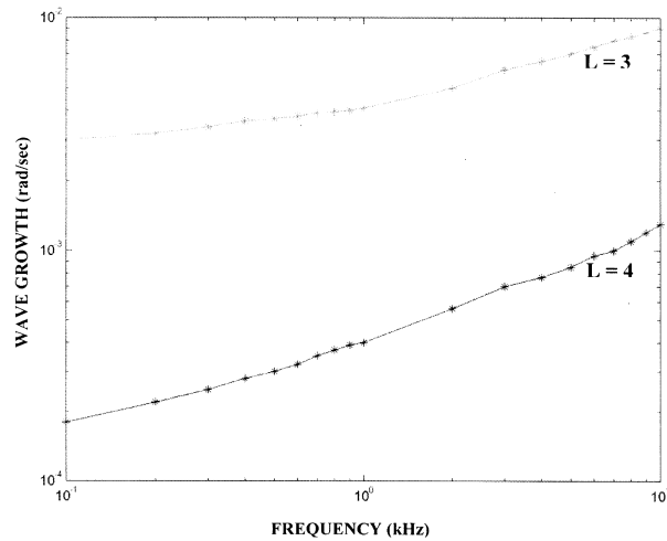
Figure 3. Variation of wave growth with frequency for different values of L .
