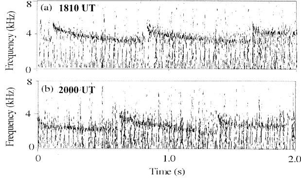
Figure 1. Typical frequency–time spectrograms of discrete VLF emissions observed at Varanasi on 29 April 1990.
