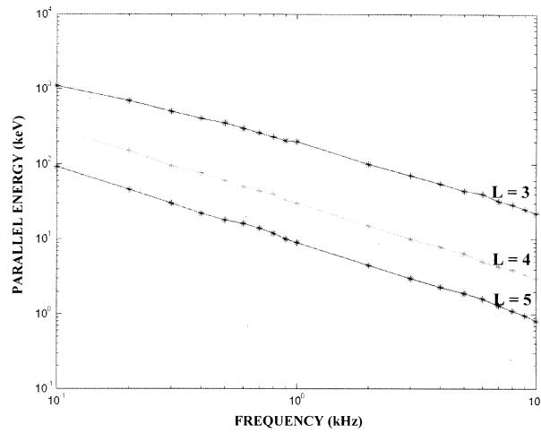
Figure 2. Variation of the parallel energy of resonating electrons with whistler wave frequency for different values of L .
