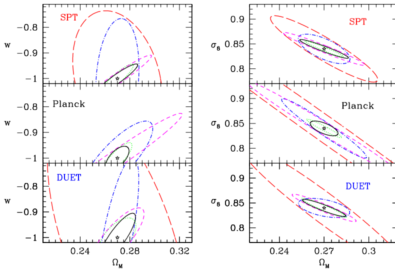
Figure 2. Left panel: 1\text{-}\sigma constraints on w and \Omega_M for an SZE SPT survey (top), SZE Planck survey (middle) and an X-ray DUET survey (bottom) for five scenarios: ‘Only Cosmology’ (dotted); constraints from dN/dz for ‘Non-Std Evol’ case (long-dashed); constraints from dN/dz + \bar{P}_{cl} , (dot-dashed); dN/dz + 100 cluster follow-up (short-dashed) and finally constraints from dN/dz + \bar{P}_{cl} + follow-up (solid). Right-panel: The corresponding constraints on \sigma_8 and \Omega_M .
