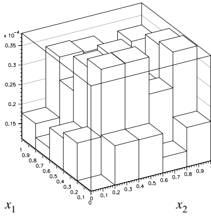
Figure 1. Doubly differential distributions in the energy fractions x_i = p_i^{\pi^\pm} / p_i^{\tau\text{-jet}} , where p_i^{\pi^\pm} is the charged pion momentum and p_i^{\tau\text{-jet}} that of the visible \tau -jet, i.e. the momentum carried away by the mesons \pi^\pm , \rho^\pm and a_1^\pm in 1-prong decays for Higgs signals and backgrounds in the \tau^+ \tau^- X channel, after the following selection cuts (at parton level): p_T(\tau\text{-jet}) > 60 \text{ GeV} , |\eta(\tau\text{-jet})| < 2.5 , \Delta\Phi(\tau\text{-jets}) < 175^\circ , \Delta R(\text{jet-jet}) > 0.4 and p_T(\text{miss}) > 40 \text{ GeV} . Normalisations are to the total cross-sections after cuts at \sqrt{s} = 14 \text{ TeV} (for M_A = M_H = 200 \text{ GeV} and \tan\beta = 30 , in the case of the signal). Bins are 0.2 units wide.
