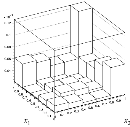
Figure 1. Doubly differential distributions in the energy fractions x_i = p_i^{\pi^\pm} / p_i^{\tau\text{-jet}} , where p_i^{\pi^\pm} is the charged pion momentum and p_i^{\tau\text{-jet}} that of the visible \tau -jet, i.e. the momentum carried away by the mesons \pi^\pm , \rho^\pm and a_1^\pm in 1-prong decays for Higgs signals and backgrounds in the \tau^+ \tau^- X channel, after the following selection cuts (at parton level): p_T(\tau\text{-jet}) > 60 \text{ GeV} , |\eta(\tau\text{-jet})| < 2.5 , \Delta\Phi(\tau\text{-jets}) < 175^\circ , \Delta R(\text{jet-jet}) > 0.4 and p_T(\text{miss}) > 40 \text{ GeV} . Normalisations are to the total cross-sections after cuts at \sqrt{s} = 14 \text{ TeV} (for M_A = M_H = 200 \text{ GeV} and \tan\beta = 30 , in the case of the signal). Bins are 0.2 units wide.
