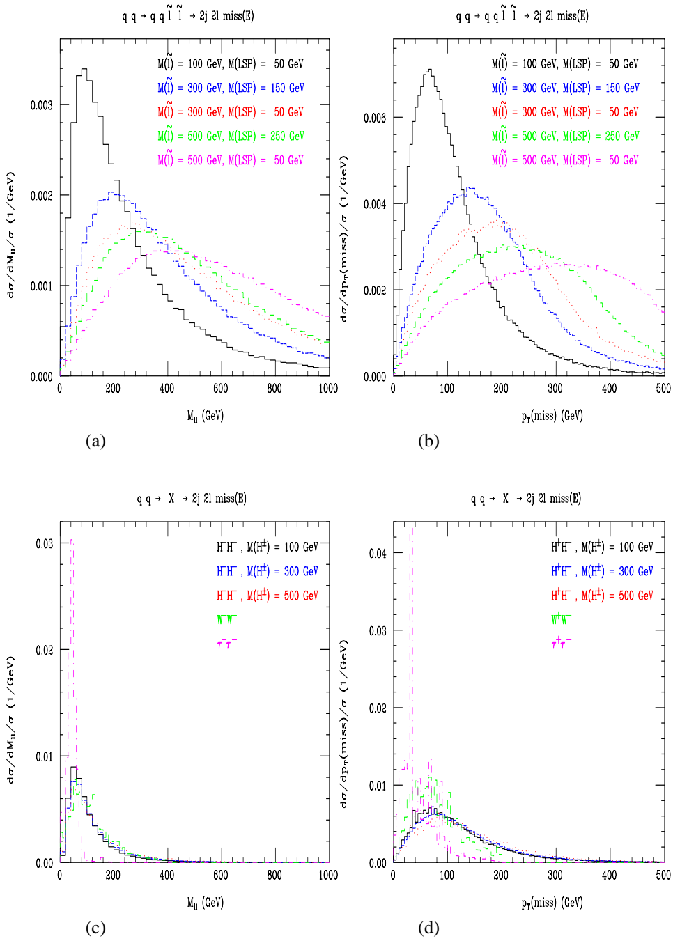
Figure 1. Invariant mass ( left ) and missing transverse momentum ( right ) distributions for the signal ( top ) and the backgrounds ( below ). Normalisations are to unity.
