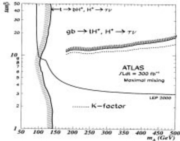
Figure 1. The ATLAS 5- \sigma discovery contours of 2HDM charged Higgs bosons for 300 fb ^{-1} of luminosity, now including the reach in the \tau\nu channel as obtained at one-loop level in QCD through overall K -factors.
