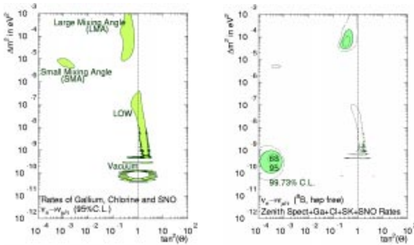
Figure 5. Left: The allowed regions in (\tan^2 \Theta, \Delta m^2) phase space remaining after the solar neutrino fluxes measured in three types of detectors are combined in a global fit. Right: The remaining phase space for oscillations after Super-K's flux and zenith angle information are added. The concentric circular regions at the lower left of this plot are a key to the contours and shading. Shaded areas in both plots are allowed at the 95% confidence level for oscillations into active neutrino species.
