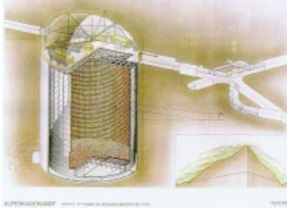
Figure 1. Cutaway view of the Super-Kamiokande detector. The detector itself stands some 42 m tall – to get a sense of the scale, consider that the tunnels shown in the drawing are large enough for full-sized trucks to drive through. The curving tunnel on the right side of the sketch contains our water purification plant; just above that is our main control room.
