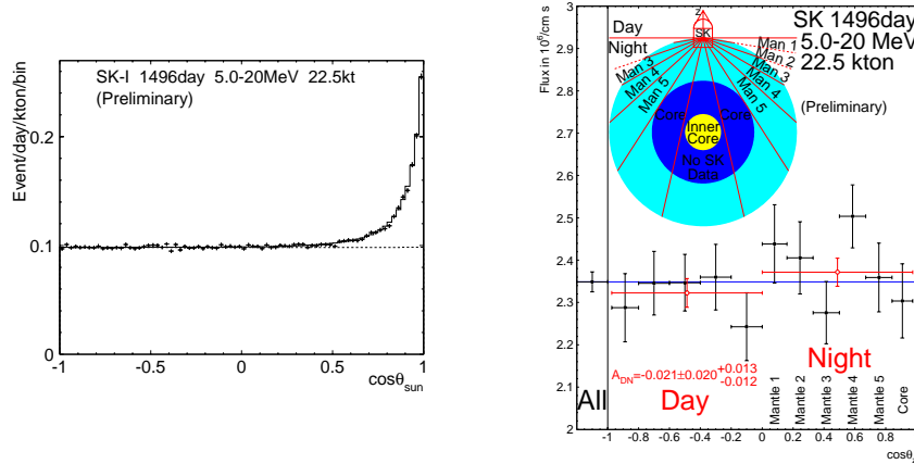
Figure 3. Left: Solar neutrino signal between 5.0 MeV and 20.0 MeV. The line is a fit to 46.5% of the BP2000 SSM. Right: Variation of the solar neutrino flux as a function of zenith angle. Both plots are the result of 1496 live days of data and a 22.5 kton fiducial volume.
