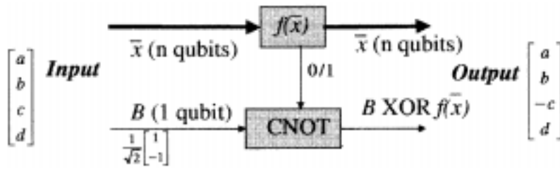
Figure 5. The above quantum mechanical circuit selectively inverts amplitudes of precisely those basis states where the function f(\bar{x}) evaluates to 1 (in the example considered, it is assumed that f(\bar{x}) is 1 in the 3rd state).
