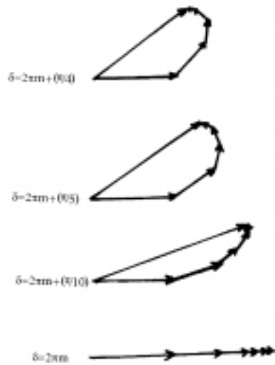
Figure 4. Geometrical construction of the resultant amplitude for dimensionless intensity 3.
