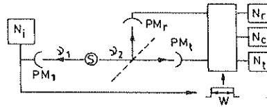
Figure 1. Study of detection correlations after a beam splitter.
