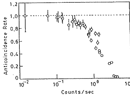
Figure 9. The anti-coincidence rate plotted against signal counts per second.
