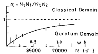
Figure 3. The anti-correlation parameter \alpha as a function of \omega N (the number of cascades excited during a gate) and the trigger rate N_1 .
