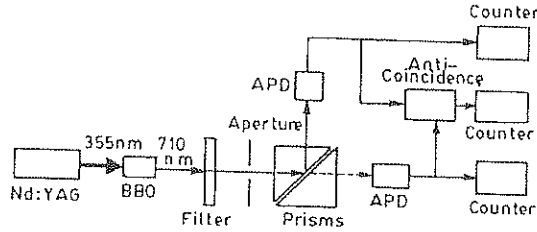
Figure 7. The anti-coincidence experiment.
