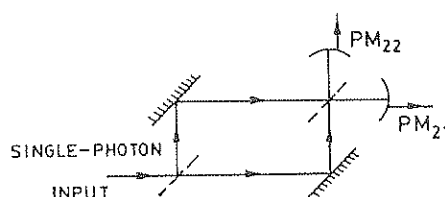
Figure 4. The Mach-Zehnder interferometer.
