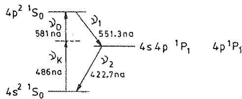
Figure 2. Two photon radiative cascade of calcium used to generate single photon wave packets.
