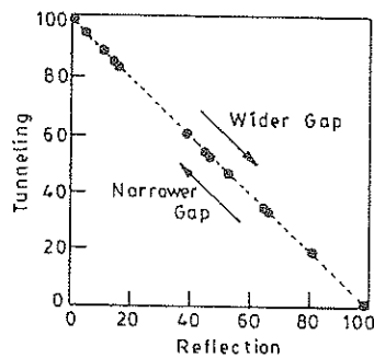
Figure 8. The relation between reflection and tunneling as the gap between the prisms is varied.
