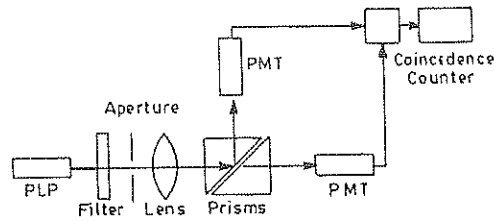
Figure 5. The coincidence experiment.
