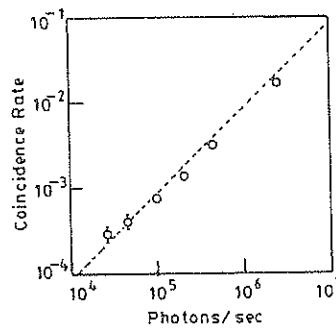
Figure 6. Coincidences as a function of singles counts per second.
