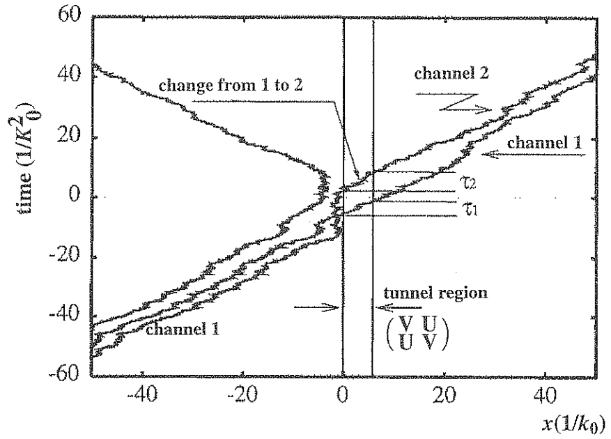
Figure 6. The three typical sample paths with the the channel coupling.
