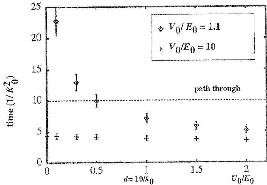
Figure 5. The mean value of \tau_p versus \frac{U_0}{E_0} (thick potential cases).
