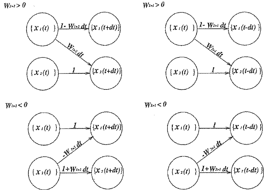
Figure 1. Schematic illustration of the “dynamical” rule for stochastic jumping process between two channels.
