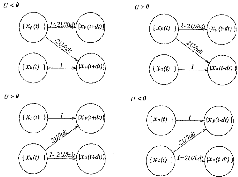
Figure 2. Schematic illustration of “dynamical” rule for stochastic jumping process between physical and unphysical sector.
