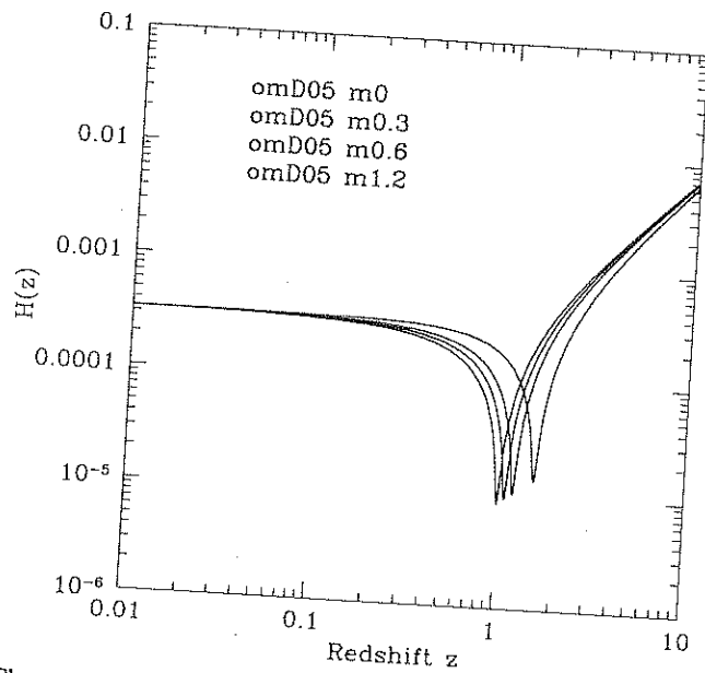
Figure 3. Hubble parameter shown as a function of cosmological redshift in a cold dark matter Universe with loitering: \Omega_{0m} = \Omega_{cdm} + \Omega_b = 0.5 , \Omega_b = 0.0125 . Four different loitering models are considered with m = 0.0, 0.3, 0.6, 1.2 .
