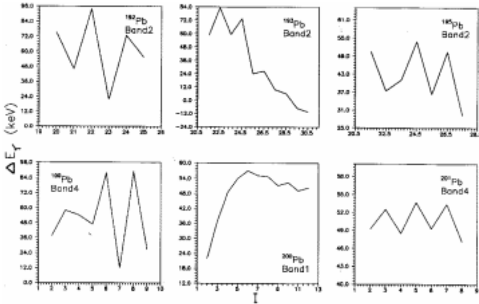
Figure 1. Signature splitting in some of the MR bands in Pb isotopes as observed in the experimental data. The spins are not known in the three cases in the bottom panels.
