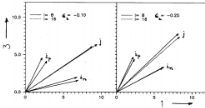
Figure 3. Geometry of particle angular momenta at I = 8 and 16 for small oblate deformation \epsilon_2 = -0.1 (left panel) and for large oblate deformation \epsilon_2 = -0.25 (right panel).
