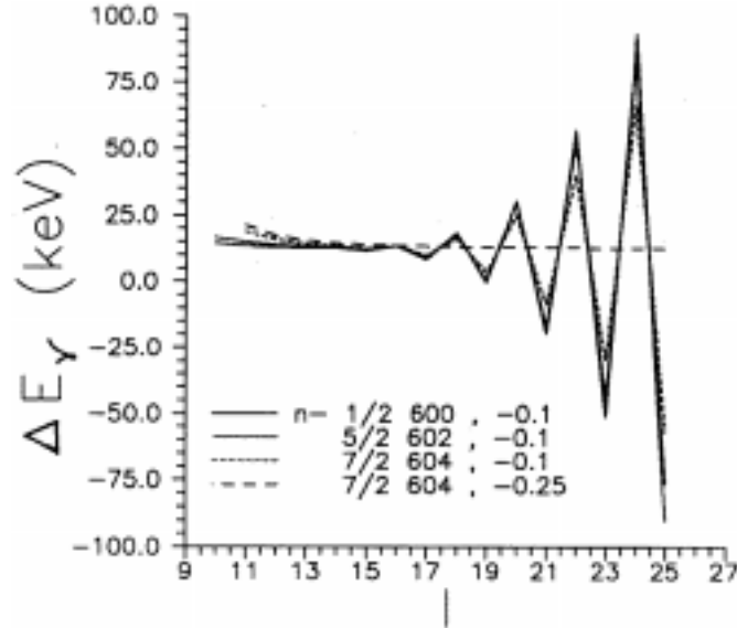
Figure 2. Staggering patterns for a DAL proton particle in 9/2[514] and RAL and mid-shell neutron hole in 1/2[600] , 5/2[602] and 7/2[604] for a small oblate deformation \epsilon_2 = -0.1 and also the result for a DAL proton particle in 9/2[514] and a neutron hole in 7/2[604] for deformation \epsilon_2 = -0.25 .
