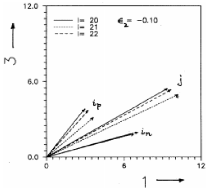
Figure 4. Geometry of particle angular momenta for three consecutive angular momenta I = 20, 21 and 22 which lie in the region of signature splitting for small oblate deformation \epsilon_2 = -0.1 .
