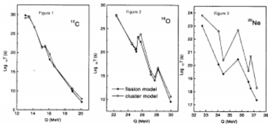
Figures 1–3. Lifetimes for the decay of lighter to heavier clusters.
