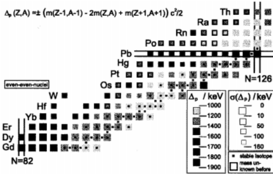
Figure 5. Proton pairing energies for even–even nuclei. The strength of the proton pairing energy \Delta_p is given by the color of the squares representing one nucleus and the error \sigma(\Delta_p) is given by the size of the squares. Masses derived from measurements at GSI are marked with a frame. The formula used is not valid to show pairing energies for the lead isotopes, as it also exhibits the larger shell effect here.
