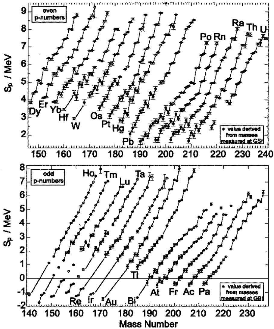
Figure 4. One proton separation energies for even (upper panel) and odd (lower panel) proton numbers. Masses derived from measurements at GSI are marked by a filled symbol.
