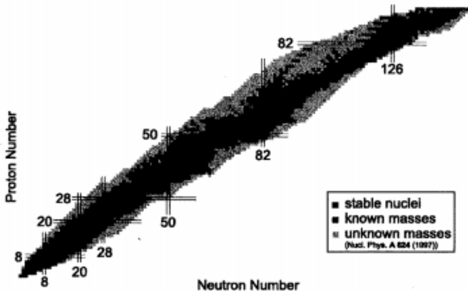
Figure 1. Chart of nuclei showing known and unknown masses up to Z = 94 .
