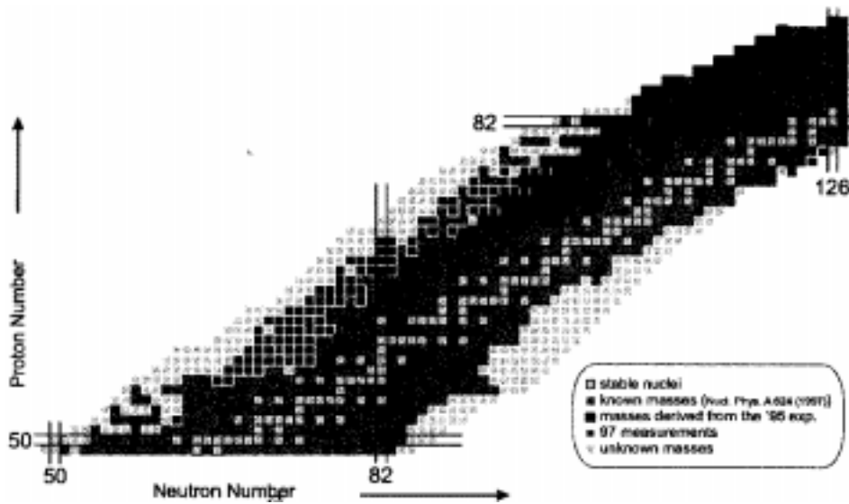
Figure 2. Range of FRS-ESR mass measurements covered in experiments with ^{209}\text{Bi} projectile fragments in 1995 and 1997. In the latter experiment we extended the measured mass surface down to cesium and also to neutron-rich fragments near the shell closures at Z = 82 and N = 126 . The marked areas of our studies represent the previously unknown masses only [7].
