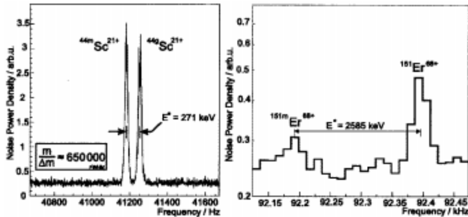
Figure 6. Mass resolved Schottky frequency spectra of bare ^{44g,m}\text{Sc} ions (ground and isomeric states separated by 271 keV, left panel) of bare ^{151g,m}\text{Er} ions (ground and isomeric states separated by 2585 keV, right panel) [7].
