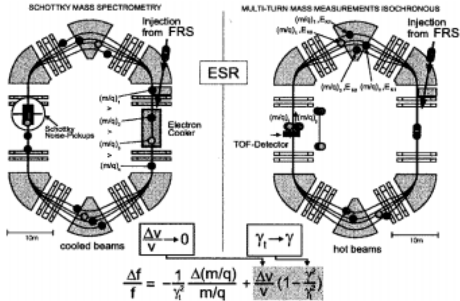
Figure 3. The mass resolution in a storage ring is given by the precision achieved for the frequency and velocity determination. \gamma is the relativistic Lorentz-factor and \gamma_t represents the reduced transition energy which characterizes the ion-optical mode of the ring. From this formula it is obvious that either cooling \Delta v/v \rightarrow 0 or the isochronous condition, \gamma \rightarrow \gamma_t , are the basis of precise mass measurements.
