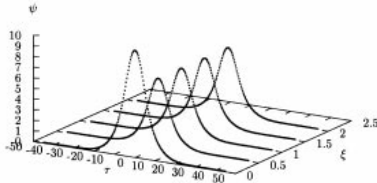
Figure 6. Intermediate down-switching of the soliton with peak intensity u_0 = 10.0 , \beta = 1.298524 \times 10^{-2} , and P_{in} = 187.8732 , belonging to the UPSB, to a soliton of peak intensity u_0 = 6.384570 ( \beta = 9.169573 \times 10^{-3} ) and P_{out} = 186.9200 , also belonging to the UPSB.
