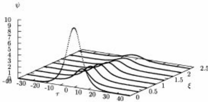
Figure 5. Down-switching of the soliton with peak intensity u_0 = 10.0 , \beta = 1.298524 \times 10^{-2} , and P_{in} = 187.8732 , belonging to the UPSB, to a soliton of the LPSB with \beta = 6.512702 \times 10^{-3} and P_{out} = 66.29978 for \kappa = 0.5 , A = 0.5 and L = 0.6366L_c .
