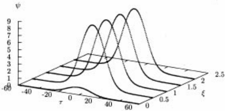
Figure 8. Up-switching of the soliton with peak intensity u_0 = 1.0 , \beta = 6.297538 \times 10^{-3} and P_{in} = 55.834690 , belonging to the LPSB, to a soliton of the UPSB with \beta = 1.170951 \times 10^{-2} and P_{out} = 186.0941 for \kappa = 0.1 , A = 1.2 and L = 0.0318L_c and \Gamma = 0.0138 .
