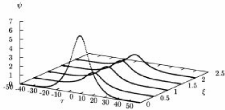
Figure 7. Final down-switching of the soliton with peak intensity u_0 = 6.384570 ( \beta = 9.169573 \times 10^{-3} ) and P_{in} = 186.9200 , to a soliton of peak intensity u_0 = 1.592637 ( \beta = 6.840451 \times 10^{-3} ) and P_{out} = 109.743300 , belonging to the LPSB.
