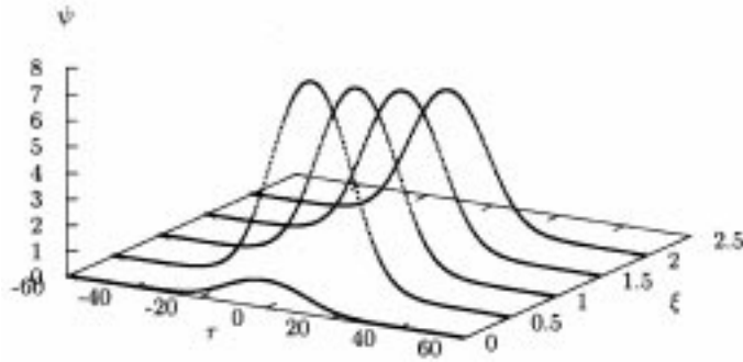
Figure 9. Up-switching of the soliton with peak intensity u_0 = 1.0 , \beta = 6.297538 \times 10^{-3} and P_{\text{in}} = 55.834690 , belonging to the LPSB, to a soliton of the UPSB with \beta = 1.058832 \times 10^{-2} and P_{\text{out}} = 184.7462 for \kappa = 0.1 , A = 1.2 and L = 0.0318L_c and \Gamma = 0.138 .
