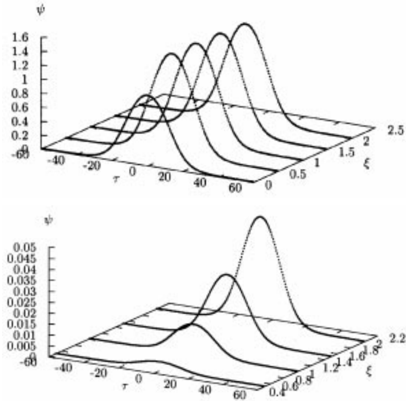
Figure 2. (a) Up-switching of the soliton with peak intensity u_0 = 1.0 , \beta = 6.297538 \times 10^{-3} and P_{in} = 55.834690 , belonging to the LPSB, to a soliton of the LPSB with \beta = 6.762296 \times 10^{-3} and P_{out} = 91.819080 for \kappa = 0.1 , A = 1.2 and L = 0.0318L_c . (b) Plot of the localized radiation that leaks into the second core during switching depicted in figure 2a.
