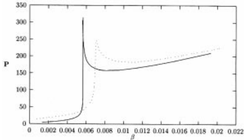
Figure 1. Plot of the soliton energy vs the nonlinear propagation constant shift \beta for \alpha = 0.08 , \delta = 5.0 and \sigma = 1.175 (solid curve), \sigma = 1.17 (dotted curve).
