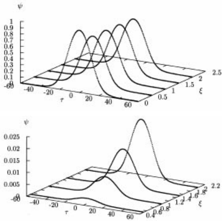
Figure 3. (a) Down-switching of the soliton with peak intensity u_0 = 1.0 , \beta = 6.297538 \times 10^{-3} , and P_{\text{in}} = 55.834690 , belonging to the LPSB, to a soliton of the LPSB with \beta = 5.891349 \times 10^{-3} and P_{\text{out}} = 44.803810 for \kappa = 0.1 , A = 0.9 and L = 0.0318L_c . (b) Plot of the localized radiation that leaks into the second core during switching depicted in figure 3a.
