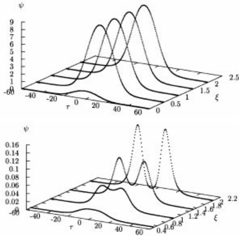
Figure 4. (a) Up-switching of the input soliton of the LPSB with peak intensity u_0 = 1.0 ( \beta = 6.297538 \times 10^{-3} , and P_{\text{in}} = 55.834690 ) to a soliton of peak intensity u_0 = 8.98 ( \beta = 1.184462 \times 10^{-2} and P_{\text{in}} = 186.367200 ), belonging to the UPSB, for \kappa = 0.1 , A = 3.0 and L = 0.0318L_c . (b) Evolution of the radiation acquired by the second core during the down-switching depicted in figure 4a.
