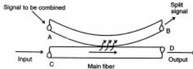
Figure 6. Four port coupler.
