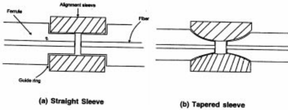
Figure 7. Connectors using butt-joint alignment designs.
