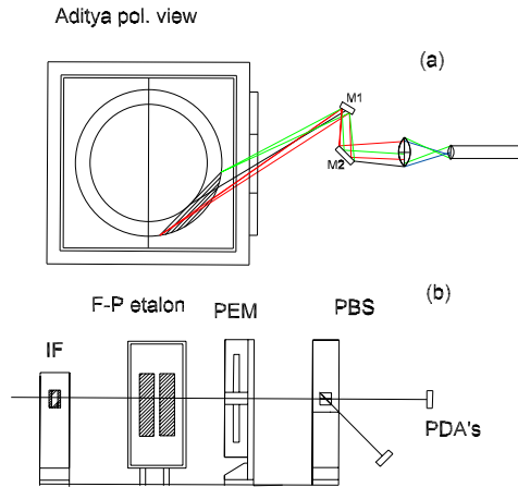
Figure 1. (a) Arrangement of the mirrors. M1, M2 are the mirrors of different dimensions. (b) Components of the Zeeman polarimeter. IF is the interference filter, F-P is the Fabry-Perot etalon, PEM is the photoelastic modulator, PBS is the polarization beam splitter and finally PDA's are the photodiode array detectors.
