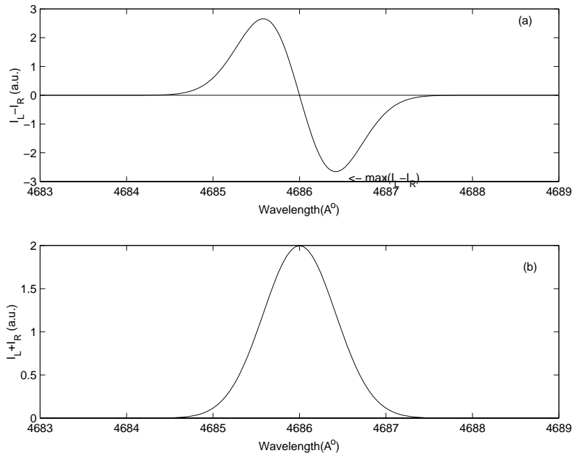
Figure 2. (a) Modulation ( I_L - I_R ) (arbitrary units) of the spectral line for ADITYA parameters. (b) Line profile signal ( I_L + I_R ) (arbitrary units).
