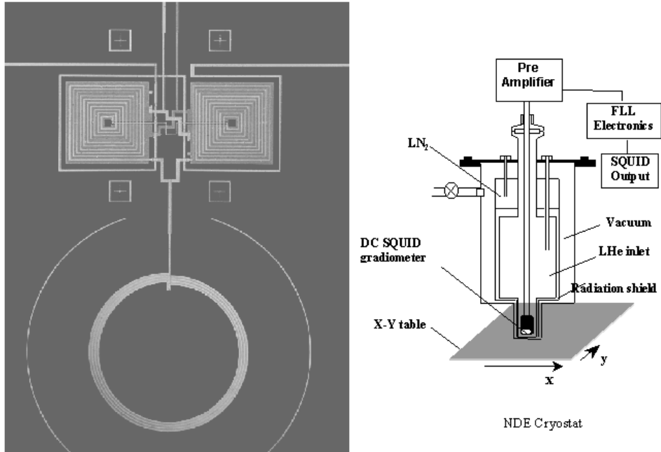
Figure 1. DC planar SQUID gradiometer with the NDE cryostat.
