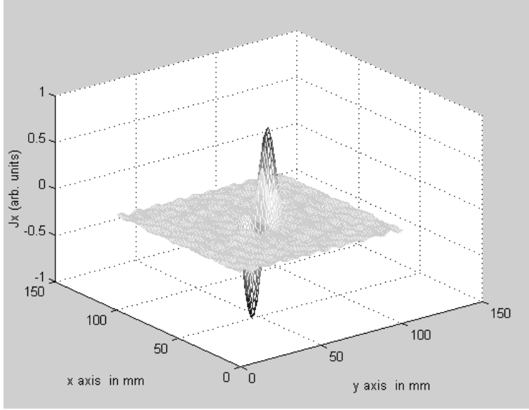
Figure 2. Inverted current density image J_x^i(x, y) .
