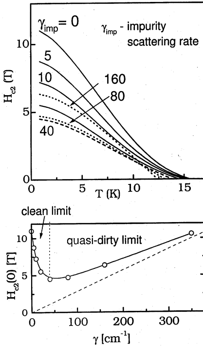
Figure 3. Temperature dependence of the upper critical field calculated within the two-band model [4] for several impurity scattering rates (upper panel). The calculated H_{c2}(0)-\gamma_{imp} dependence in the lower panel illustrates the transition from the clean to the dirty limit. Dotted line: H_{c2}(0)-\gamma_{imp} dependence within the dirty limit.
