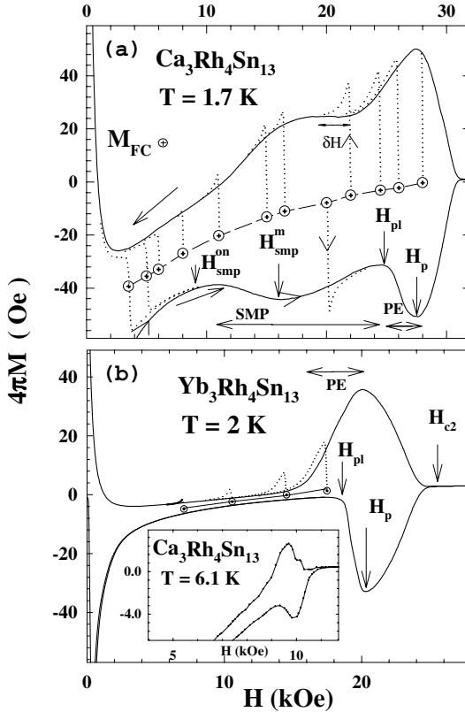
Figure 2. M - H loops for \text{CaRhSn} (a) and \text{YbRhSn} (b). Inset in panel (b) shows the M - H loop in \text{CaRhSn} at 6.1 K, where only the PE is evident.
