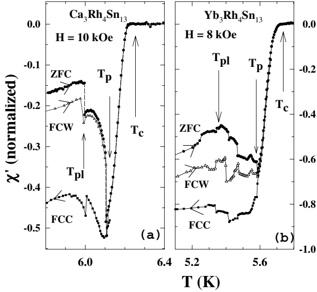
Figure 1. Isofield \chi'_{ac}(T) in CaRhSn (a) and YbRhSn (b) for three sample histories (ZFC, FCW and FCC).
