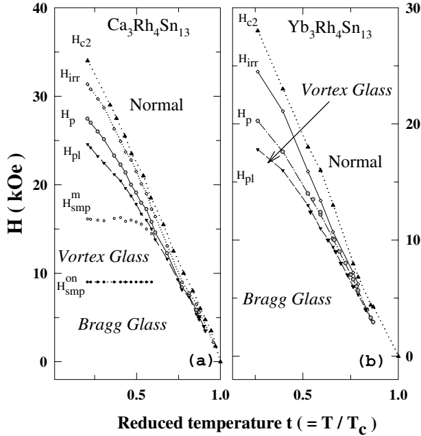
Figure 3. Vortex phase diagrams for CaRhSn (a) and YbRhSn (b), respectively.
