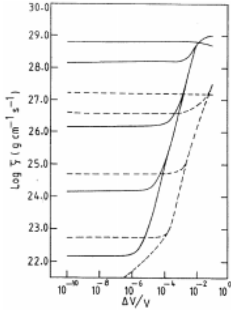
Figure 2. Graph of viscosity vs. (\Delta v/v) . Solid curves have the same meaning as in figure 1 for temperatures 10^{-5}, 10^{-4}, 10^{-3}, 10^{-2} and 10^{-1} MeV from bottom to top. The dashed lines are from Ashok Goyal et al [12] for m_s = 80, \alpha_c = 0.1 and \tau = 10^{-3} for same temperatures from bottom to top.
