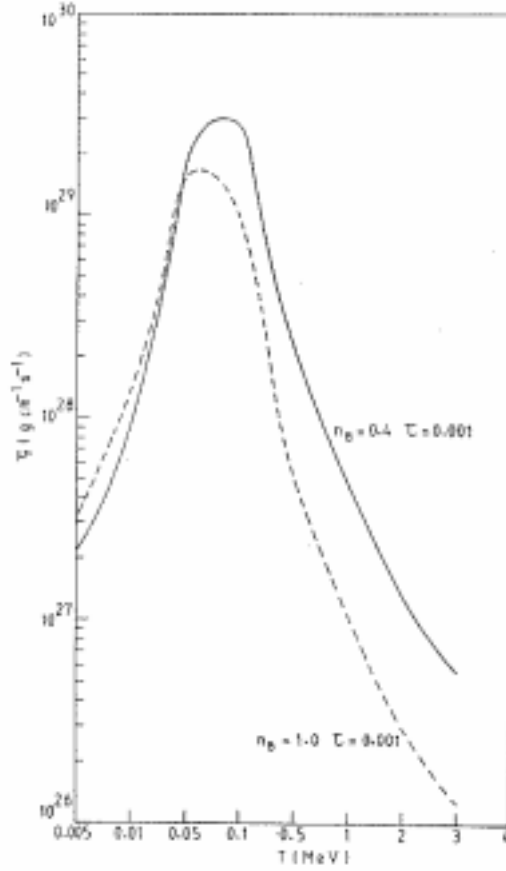
Figure 6. Variation of bulk viscosity with temperature for c = 75 , m_{s0} = 140 , \tau = 10^{-3} . The solid curve is for n_b = 0.4 \text{ fm}^{-3} and the dashed curve is for n_b = 1.0 \text{ fm}^{-3} .
