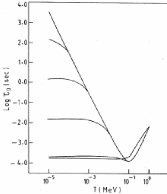
Figure 5. Plot of damping time vs. temperature for a 1.4 M_\odot strange star for c = 75 \text{ MeV fm}^{-3} , m_{s0} = 140.0 \text{ MeV} , \tau = 10^{-3} \text{ s} . Curves from bottom to top correspond to perturbation amplitudes (\Delta v/v) = 10^{-1}, 10^{-2} , ending at 10^{-6} .
