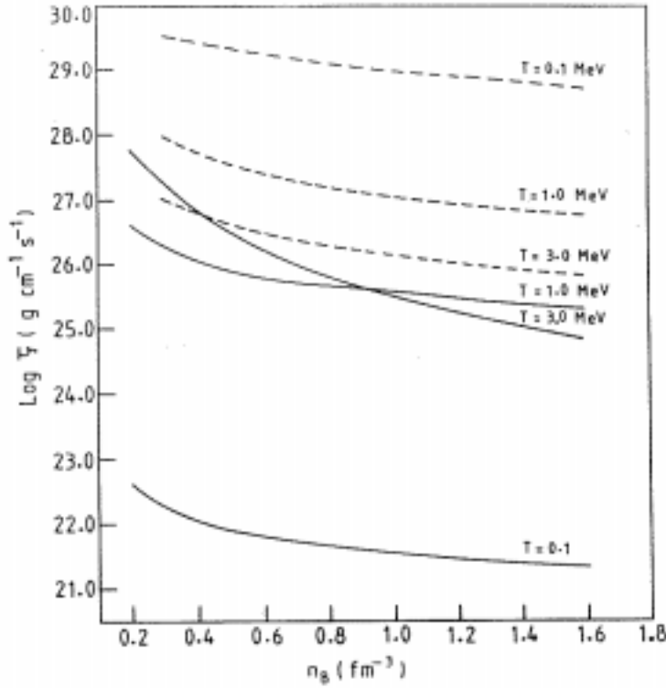
Figure 4. Bulk viscosity as a function of baryon density for c = 75.0, m_{s0} = 140.0, \tau = 10^{-3} for leptonic (solid) and non-leptonic (dashed) processes.
