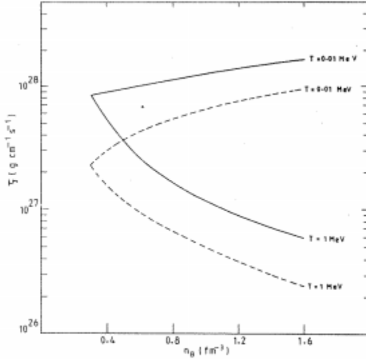
Figure 3. Bulk viscosity as a function of baryon density at T = 10^{-2} and T = 1 MeV. Solid curves are for c = 75 , m_{s0} = 140 , \tau = 10^{-3} s. The dashed curves are from ref. [12].
