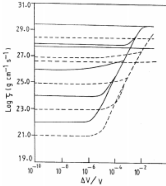
Figure 1. Bulk viscosity as a function of relative perturbation ( \Delta v/v ) for n_B = 0.4 \text{ fm}^{-3} , \tau = 10^{-3} \text{ s} for temperatures 10^{-5}, 10^{-4}, 10^{-3}, 1, 10^{-2}, 10^{-1} from bottom to top. Solid curves are for c = 75.0 \text{ MeV fm}^{-3} , m_{s0} = 14.0 \text{ MeV} and dashed curves are for c_s = 95 and m_{s0} = 55 .
