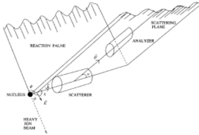
Figure 1. Schematic diagram for the emission and scattering of the initial polarized photons from aligned nuclei.
