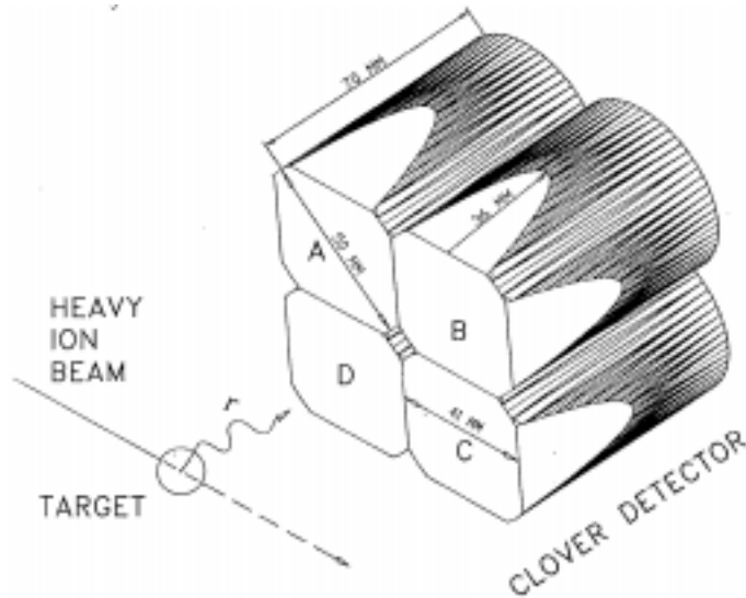
Figure 2. Schematic diagram of a clover detector consisting of four coaxial HPGe crystals. The letters A, B, C and D are used to label the different segments of the clover as used in the text.
