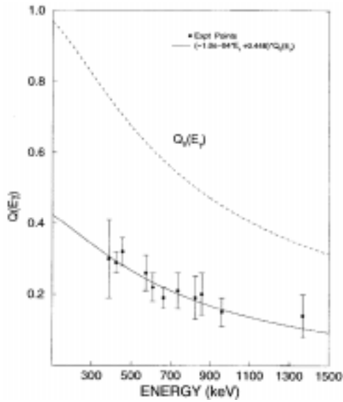
Figure 3. Polarization sensitivity of the clover detector measured as a function of gamma ray energy. The dotted line is the sensitivity for the point scatterer and analyser. Solid curve is obtained by fitting experimental data to eq. (9) with D = 0.446 and C = -0.0001 \text{ keV}^{-1} .
