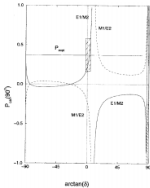
Figure 4. Calculated polarization P_{\text{cal}}(90^\circ) for the 1117 keV ( 23/2^- \rightarrow 21/2^+ ) in ^{99}\text{Rh} plotted as a function of \arctan \delta assuming E1+M2 and M1+E2 multipolarities. The experimentally measured polarization is shown by the shaded region. The intercept with E1+M2 curve gives \delta = 0.015(55) in agreement with a small a_4 value in the angular distribution measurement.
