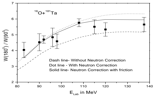
Figure 2. Fission fragment anisotropies for the system ^{16}\text{O} + ^{181}\text{Ta} .
