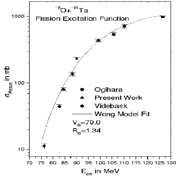
Figure 1. Fission excitation function for ^{16}\text{O} + ^{181}\text{Ta} .
