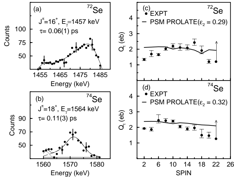
Figure 1. (a) and (b) show the lineshapes of transitions from 16^+ state of ^{72}\text{Se} and 18^+ state of ^{74}\text{Se} , respectively. (c) and (d) depict the comparison of experimental and calculated Q_t values for ^{72,74}\text{Se} .
