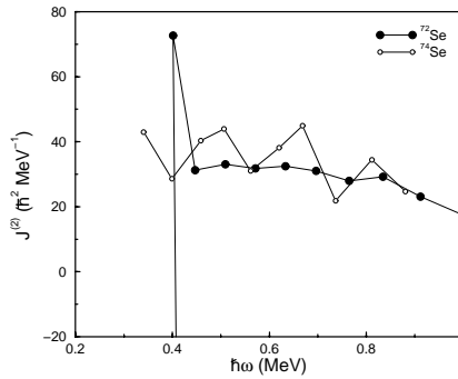
Figure 2. Comparison of J^{(2)} values for the yrast positive parity bands of ^{72,74}\text{Se} .
