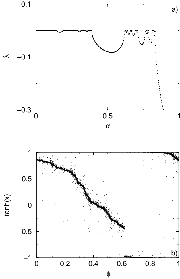
Figure 2. The Fibonacci chain, where \omega = (\sqrt{5} - 1)/2 . (a) Variation of the Lyapunov exponent with forcing parameter \alpha . Each zero of the Lyapunov exponent corresponds to an eigenstate in the quantum system, and a critical SNA in the classical system. (b) A typical SNA in this system, for E = 0 , \alpha = 0.8326745 . Note that the variable plotted on the ordinate is \tanh x rather than x ; this is merely for convenience.
