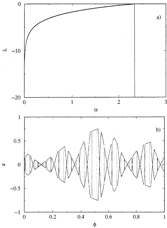
Figure 1. The piecewise linear system with \omega = (\sqrt{5} - 1)/2 . Plot of (a) the Lyapunov exponent as a function of the parameter \alpha , showing the blowout bifurcation at \alpha \approx 2.33 , above which the Lyapunov exponent \rightarrow -\infty , and (b) the strange nonchaotic attractor for \alpha = 2.5
