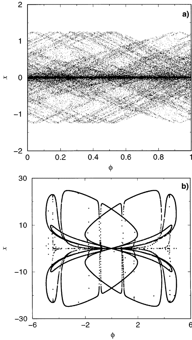
Figure 3. (a) SNA in the system eq. (20) where the driving is no longer quasiperiodic. The parameters are \alpha = 2.5 , \omega is the golden mean ratio. (b) SNA in the system given by eqs (23)–(25), where the map governing the \phi dynamics itself has SNA dynamics. The parameters \alpha and \beta are both 2.5.
