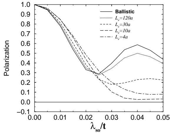
Figure 10. Polarization as a function of Rashba spin-orbit coupling parameter. Different curves correspond to different mean free path as shown in the figure. The system size is 80 \times 80 .
