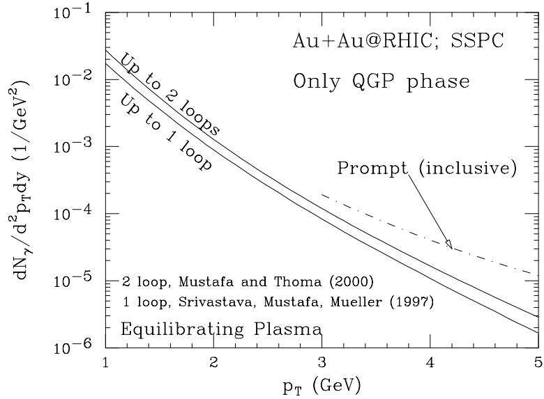
Figure 9. The production of single photons at RHIC energies, for a chemically equilibrating plasma. The initial conditions are taken from the SSPC model (table 1). The contribution from only the quark matter are shown.
