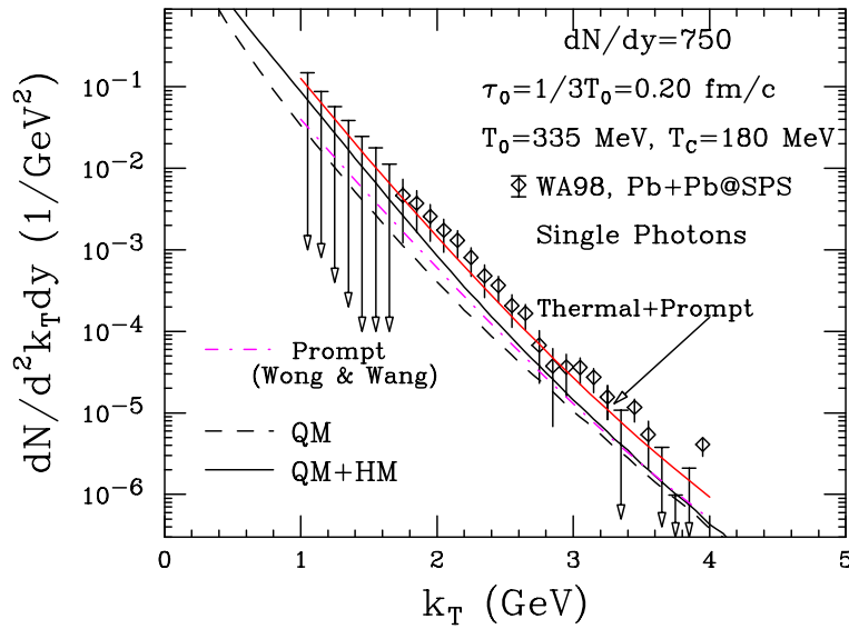
Figure 3. Single photon production in Pb+Pb collision at the CERN SPS. A chemically and thermally equilibrated quark-gluon plasma is assumed to be formed at \tau_0 = 1/3T_0 which expands, cools, enters into a mixed phase and undergoes freeze-out from a hadronic phase. QM stands for radiations from the quark matter in the QGP phase and the mixed phase. HM, likewise denotes the radiation from the hadronic matter in the mixed phase and the hadronic phase. Prompt photons are estimated using NLO pQCD with the inclusion of intrinsic k_T of partons (Wong and Wang [21]). The (tail) ends of the arrows denote the upper limit of the production at 90% confidence limit.
