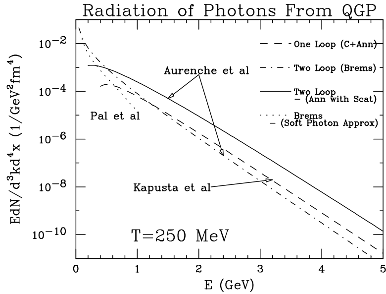
Figure 2. Rate of emission of photons from quark-gluon plasma due to various mechanisms.
