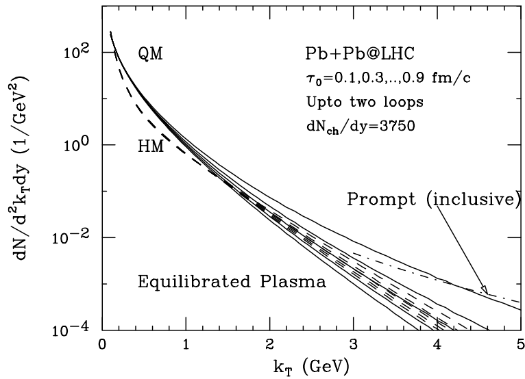
Figure 8. The production of single photons at LHC energies. The initial time at which the plasma is formed in thermal and chemical equilibrium is changed to see when should the radiation from the quark matter outshine that from the hadronic matter.
