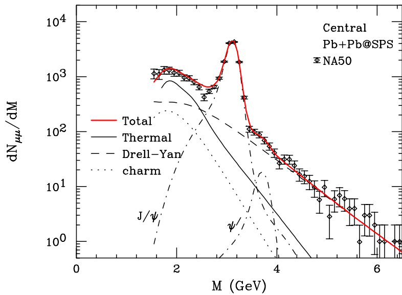
Figure 5. The invariant mass distribution of dilepton production in NA50 experiment [4].
