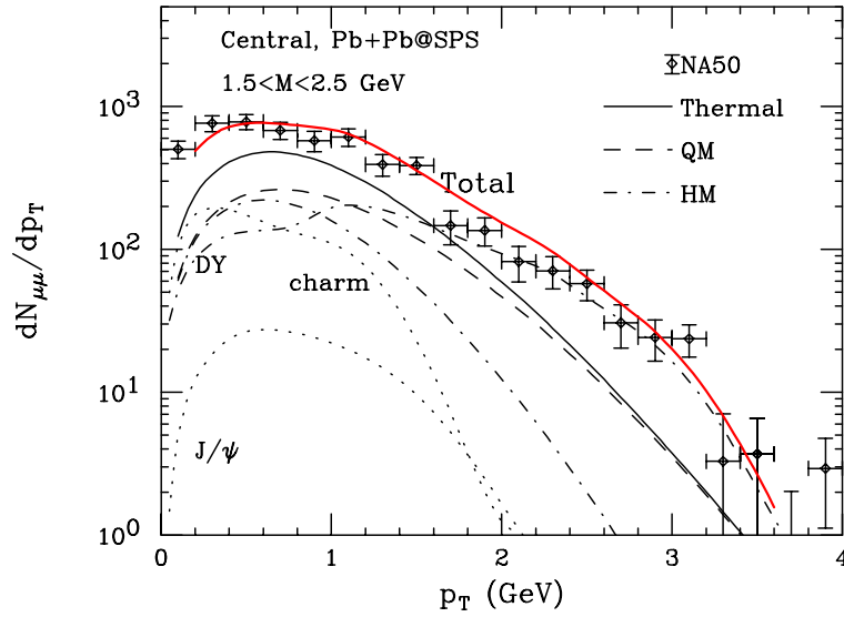
Figure 6. The p_T distribution of dileptons produced in central collision of lead nuclei.
