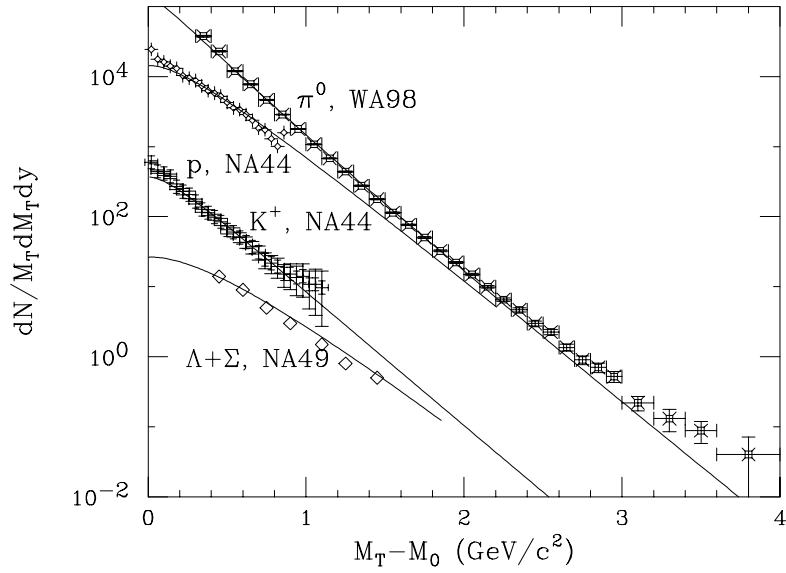
Figure 4. Transverse momentum spectra of neutral pions, protons, kaons and \Sigma + \Lambda in central collisions of lead nuclei at CERN SPS.
