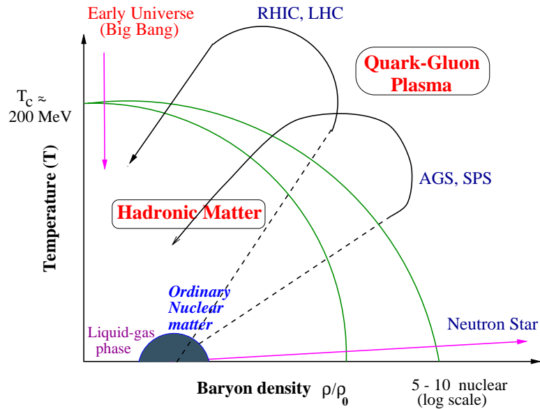
Figure 1. A schematic view of the phase diagram of hot hadronic and quark matter.
