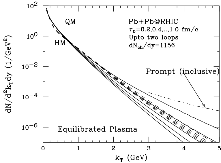
Figure 7. The production of single photons at RHIC energies. The initial time at which the plasma is formed in thermal and chemical equilibrium is changed to see when should the radiation from the quark matter outshine that from the hadronic matter.
