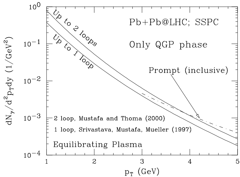
Figure 10. The production of single photons at LHC energies, for a chemically equilibrating plasma. The initial conditions are taken from the SSPC model (table 1). The contribution from only the quark matter are shown.
