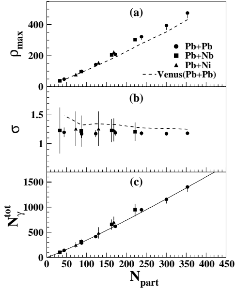
Figure 2. (a) Pseudorapidity density ( \rho_{\max} ), (b) width of the pseudorapidity distributions ( \sigma ), and (c) integrated values of number of photons ( N_{\gamma}^{\text{tot}} ), as functions of the number of participant nucleons at different centrality bins for Pb induced reactions on Ni, Nb, and Pb targets at 158 A GeV. The solid line in (c) is a power-law fit to the data, which yields the value of the exponent, \alpha = 1.12 \pm 0.03 .
