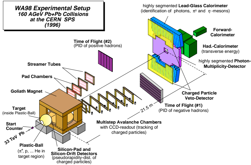
Figure 1. Layout of the WA98 experiment. The photon multiplicity detector was an Indian contribution.
