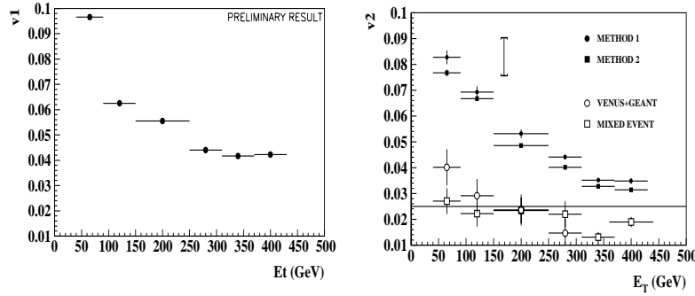
Figure 3. Left: Directed flow component v_1 as a function of centrality; right: elliptic flow component v_2 as a function of centrality.
