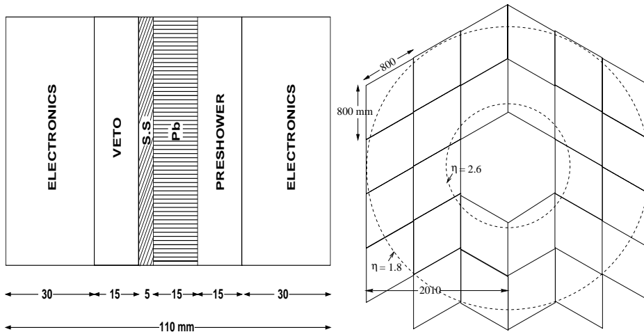
Figure 7. Left: Cross-section of the PMD (schematic only) showing the veto plane, lead converter and the preshower plane. SS is the support plate on which lead plates and chambers will be mounted. Right: The layout and the pseudorapidity coverage. Each rhombus denotes a supermodule of side 80 cm containing 72 \times 72 hexagonal cells. The detector has a vertical axis of symmetry and the two halves can be opened independently.
