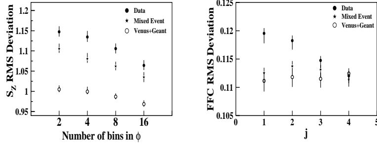
Figure 4. Left: S_z rms deviation; right: FFC rms deviation.
