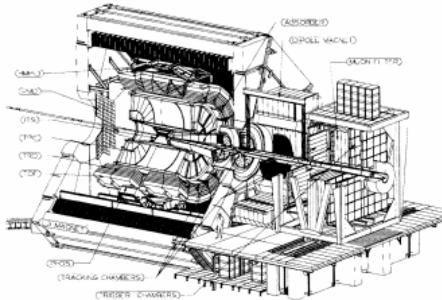
Figure 6. Layout of the ALICE experiment.
