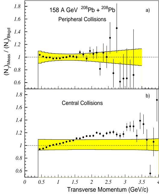
Figure 5. Preliminary result on direct single photons from WA98 experiment.
