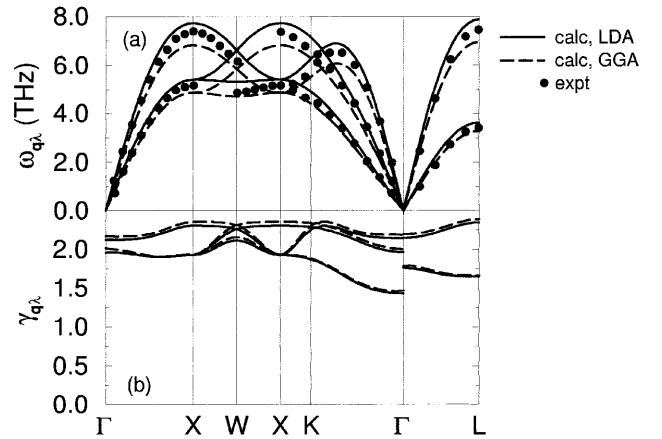
Figure 1. Dispersion along high-symmetry directions of the Brillouin zone of (a) phonon frequencies, \omega_{\mathbf{q}\mathbf{l}} and (b) mode Grüneisen parameters, g_{\mathbf{q}\mathbf{l}} , evaluated at the static lattice constant. The solid and dashed lines are the results obtained using LDA and GGA, respectively, the dots are experimental points at room temperature (Drexel 1972; Nilsson and Rolandson 1973; Lynn et al 1973). Note that the discrepancy between LDA and GGA results is much less in (b) than in (a).
