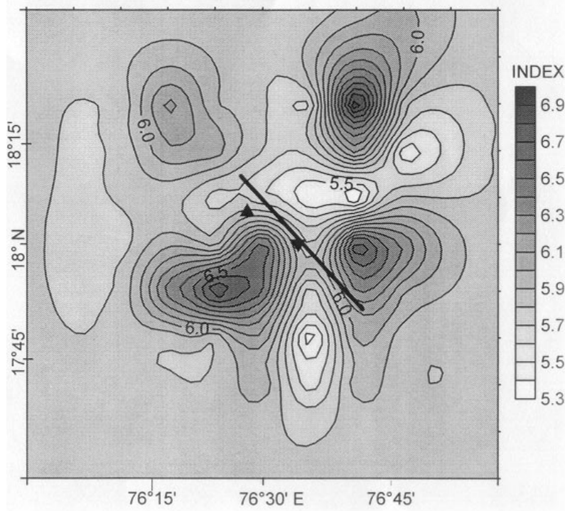
Figure 7. A horizontal slice through the estimated 3D velocity structure of the area at the depth level 6 km. The main shock focus (both the USGS and NGRI estimates) is located at the junction of a high velocity and a low velocity zone. Index shows the velocity values in km/s. The NGRI and USGS estimates of the main shock are shown by filled inverted and upright triangles, respectively. The fault plane orientation as estimated by HRV (after Baumbach et al 1994) is shown through the NGRI estimate of main shock.
