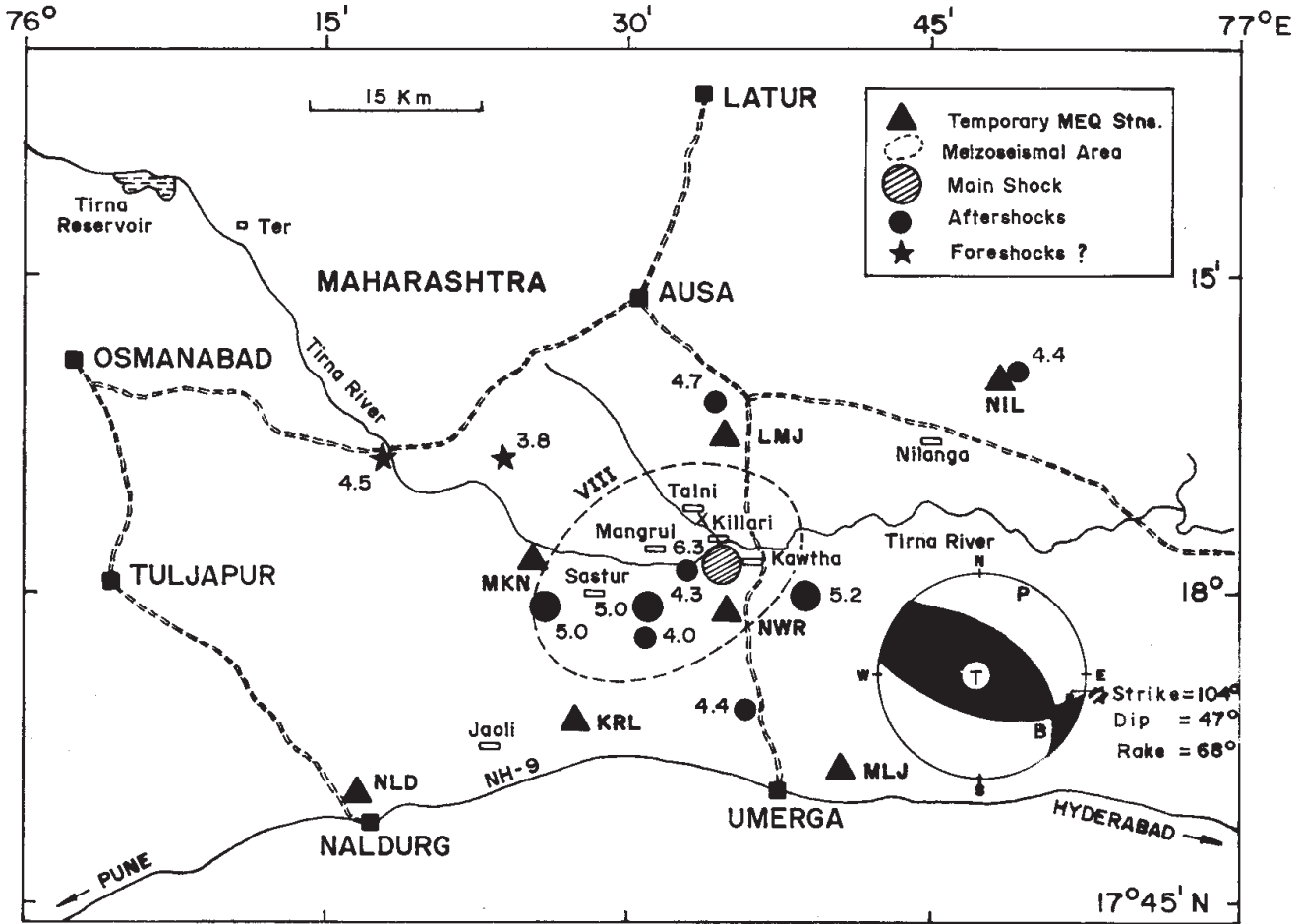
Figure 1. Map showing the main shock epicentre (NGRI), meizoseismal zone (intensity VIII) and the fault plane (CMT) solution of the main shock (after Kayal 2000).
