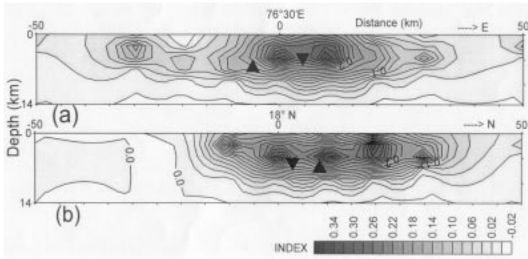
Figure 11. E-W (a) and N-S (b) sections through the center ( 18^{\circ}\text{N} , 76.5^{\circ}\text{E} , shown as 0) of the study area showing variations of resolution for P wave velocity. The resolution values are shown along the contours and also in the index. The NGRI and USGS estimates of the main shock are shown by filled inverted and upright triangles respectively.
