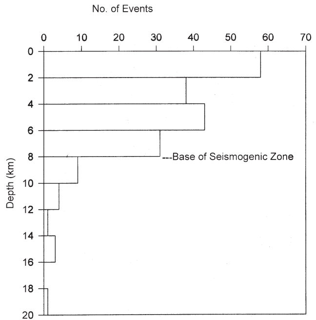
Figure 8. Plot showing the number of events versus depth. The base of the seismogenic zone is at 8 km (see text).
