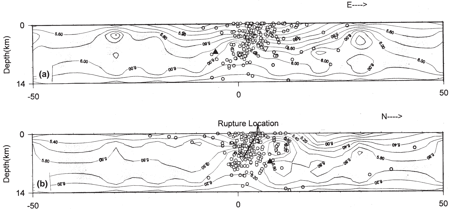
Figure 6. E-W (a) and N-S (b) depth sections of the aftershocks (figure 5), which are relocated by the 3-D simultaneous inversion technique. The sections incorporate the velocity perturbations (thin lines) obtained by the inversion technique along 76.5^\circ E and 18^\circ N respectively. The NGRI and USGS estimates of the main shock are shown by inverted open and filled triangles, respectively. Aftershocks are shown by open circles.
