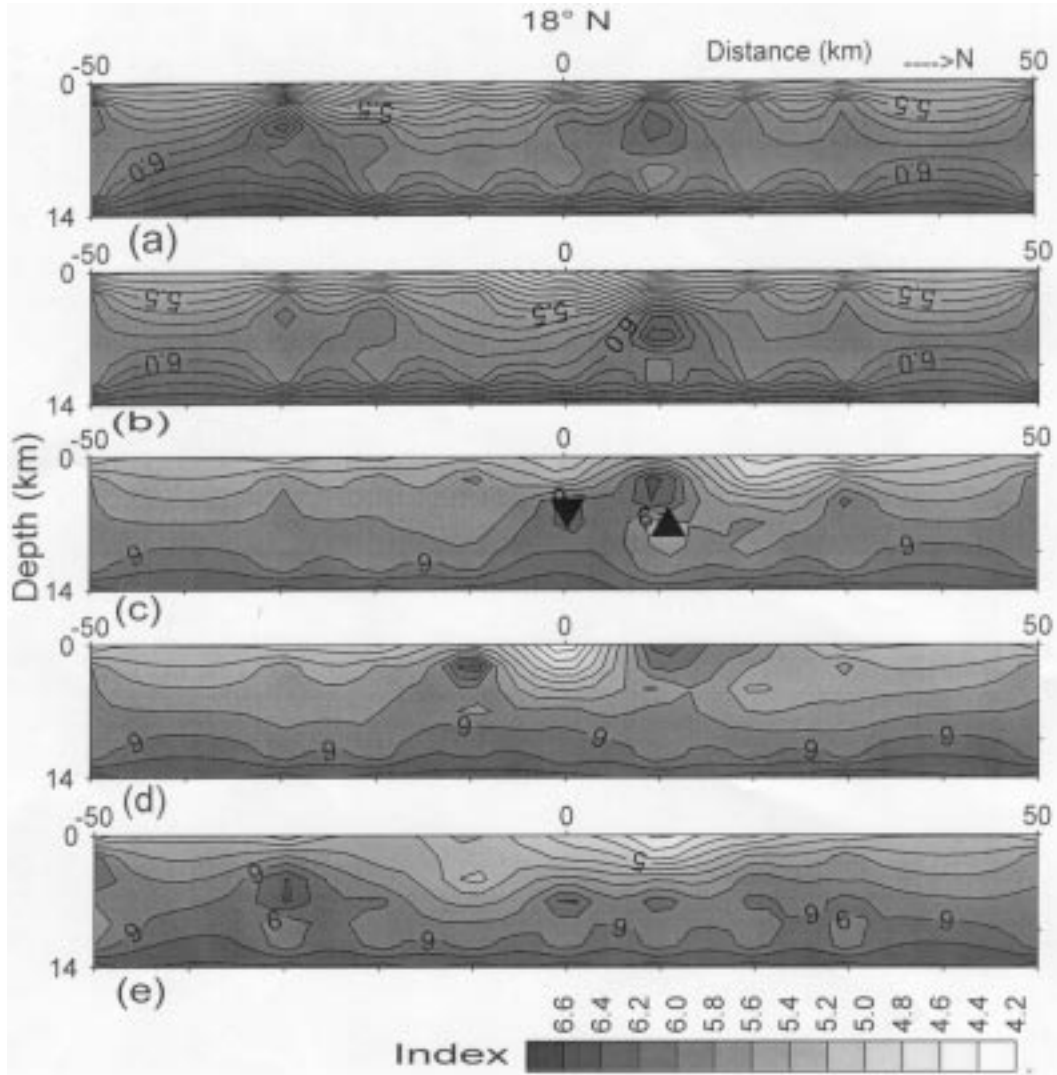
Figure 10. N-S oriented vertical slices through the estimated 3-D velocity structure of the study area. Contoured values of velocities are in km/s. The slices are 10 km apart; figure 10(a) is the easternmost and figure 10(e) is the westernmost slice respectively. The central slice (figure 10c) is along longitude 76.5^\circ E. The centre of the section shown by 0 is at 18^\circ N. Index shows velocity values in km/s. The NGRI and USGS estimates of the main shock are shown by filled inverted and upright triangles respectively.
