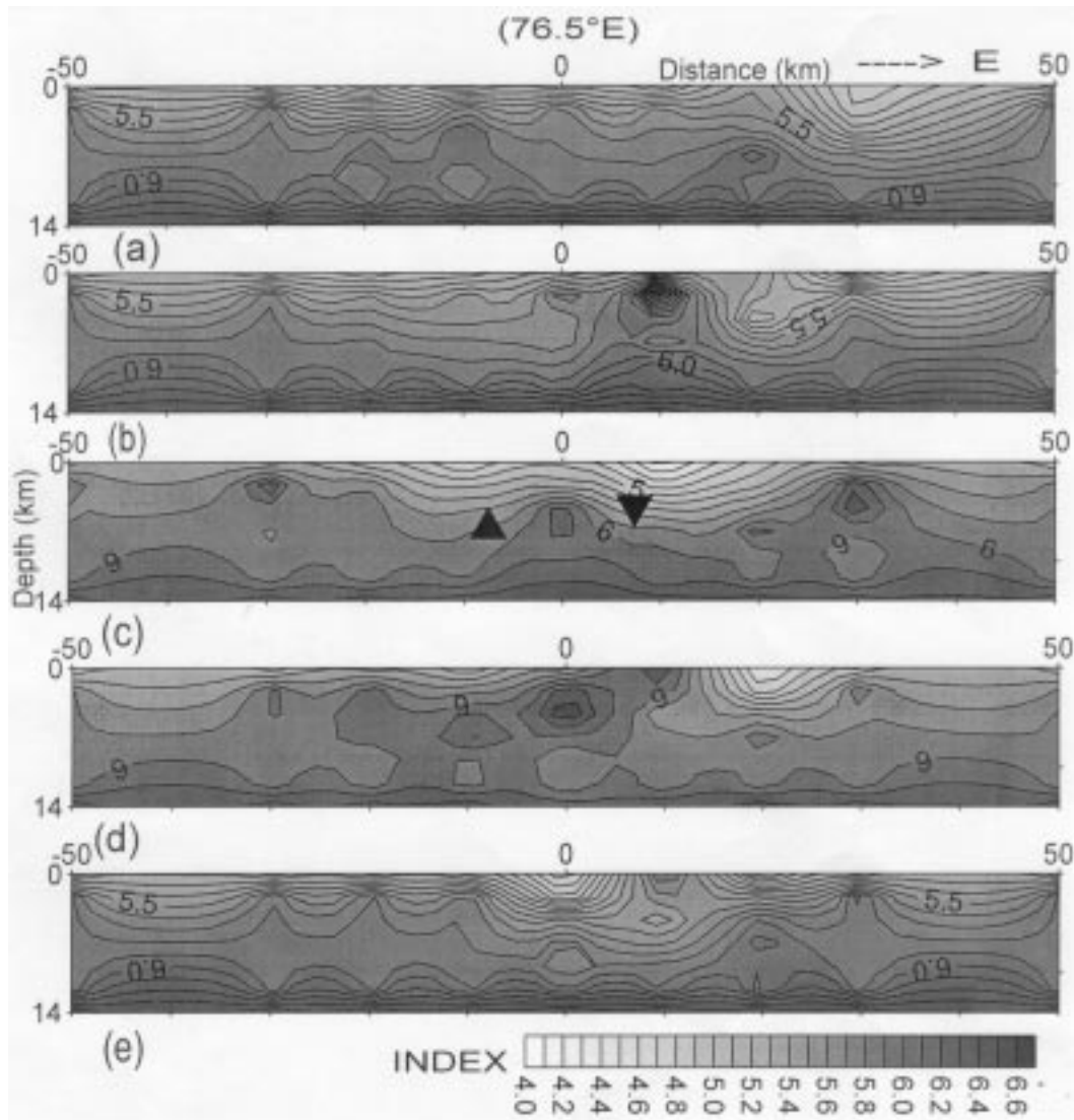
Figure 9. E-W oriented vertical slices through the estimated 3-D velocity structure of the study area. Contoured values of velocities are in km/s. The slices are 10 km apart; figure 9(a) is the northernmost and figure 9(e) is the southernmost slice, respectively. The central slice (figure 9c) is along latitude 18° N. The centre of the section shown by 0 is at 76.5° E. Index shows velocity values in km/s. The NGRI and USGS estimates of the main shock are shown by filled inverted and upright triangles respectively.
