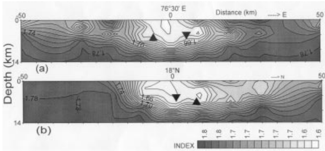
Figure 13. E-W (a) and N-S (b) sections through the center ( 18^\circ N, 76.5^\circ E, shown as 0) of the study area showing variation of V_P/V_S . The V_P/V_S values are shown along the contours and also in the index. The NGRI and USGS estimates of the main shock are shown by filled inverted and upright triangles respectively.
