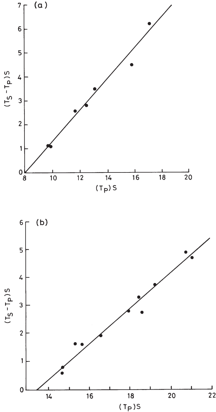
Figure 2. Examples of Wadati diagrams showing good fit of the data.
