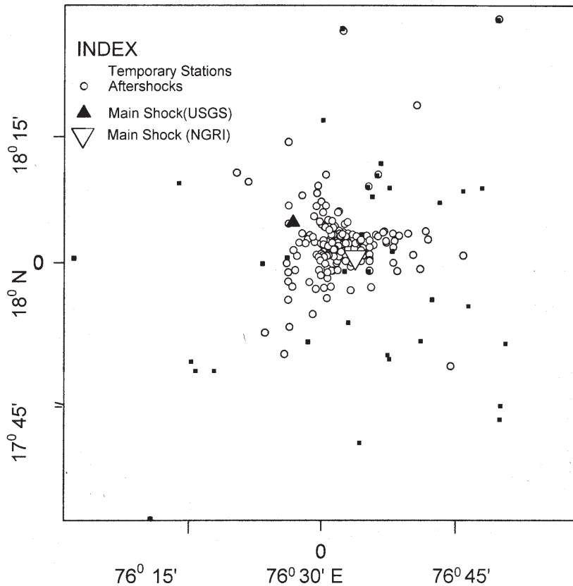
Figure 3. Map showing initial estimates of the aftershock epicenters using a 1-D velocity model and HYPO-71 program (see text). The NGRI and USGS estimates of the main shock are shown by inverted open and filled triangles, respectively.
