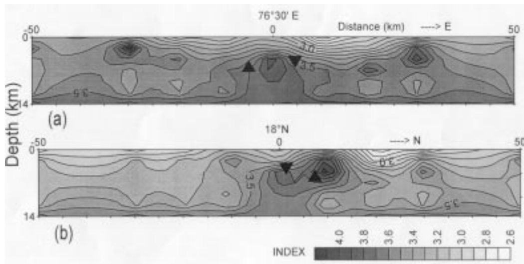
Figure 12. E-W (a) and N-S (b) sections through the center ( 18^{\circ}\text{N} , 76.5^{\circ}\text{E} , shown as 0) of the study area showing variations of S -wave velocity. The velocity values are shown along the contours in km/s and also in the index. The NGRI and USGS estimates of the main shock are shown by filled inverted and upright triangles respectively.
