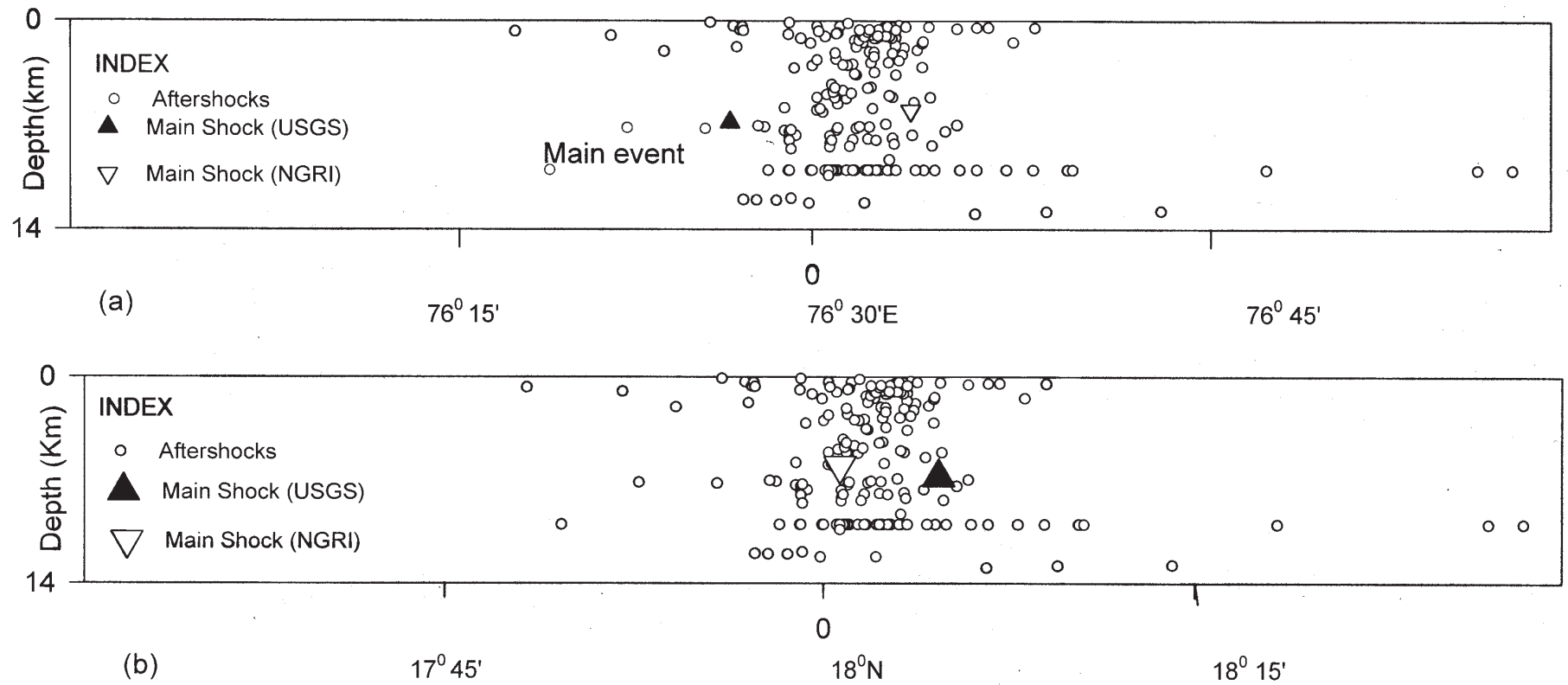
Figure 4(a) E-W and (b) N-S depth sections of the aftershocks in figure 3. Many aftershocks are located with fixed depth at 10 km by the HYPO-71 program. The NGRI and USGS estimates of the main shock are shown by inverted open and filled triangles, respectively.
