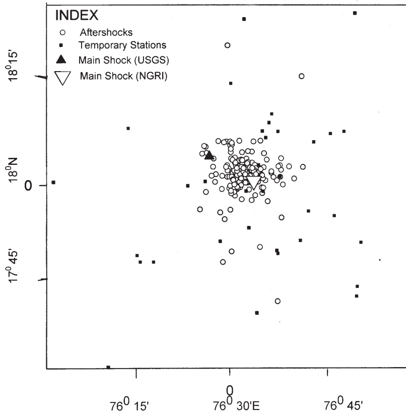
Figure 5. Map showing the relocated epicentres of the aftershocks using the 3-D simultaneous inversion technique. The NGRI and USGS estimates of the main shock are shown by inverted open and filled triangles, respectively.
