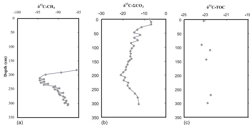
Figure 3. Depth profiles of (a) \delta^{13}\text{C}-\text{CH}_4 , (b) \delta^{13}\text{C}-\Sigma\text{CO}_2 and (c) \delta^{13}\text{C}-\text{TOC} .
