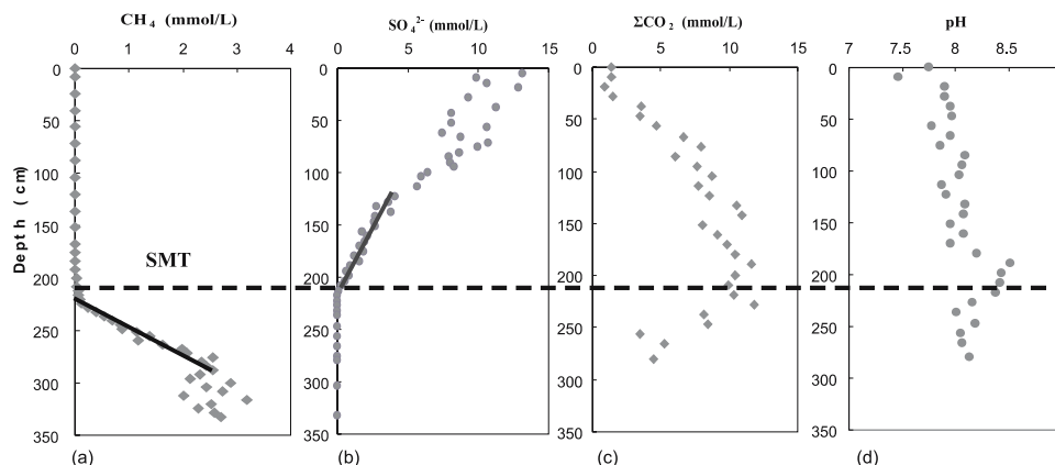
Figure 2. Pore water profiles of (a) methane, (b) sulfate, (c) total dissolved carbon dioxide concentrations ( \Sigma\text{CO}_2 ) and (d) pH (the hatched bar marks the sulfate-methane transition zone, and the gradients used for diffusive flux calculation are indicated by the solid lines).
