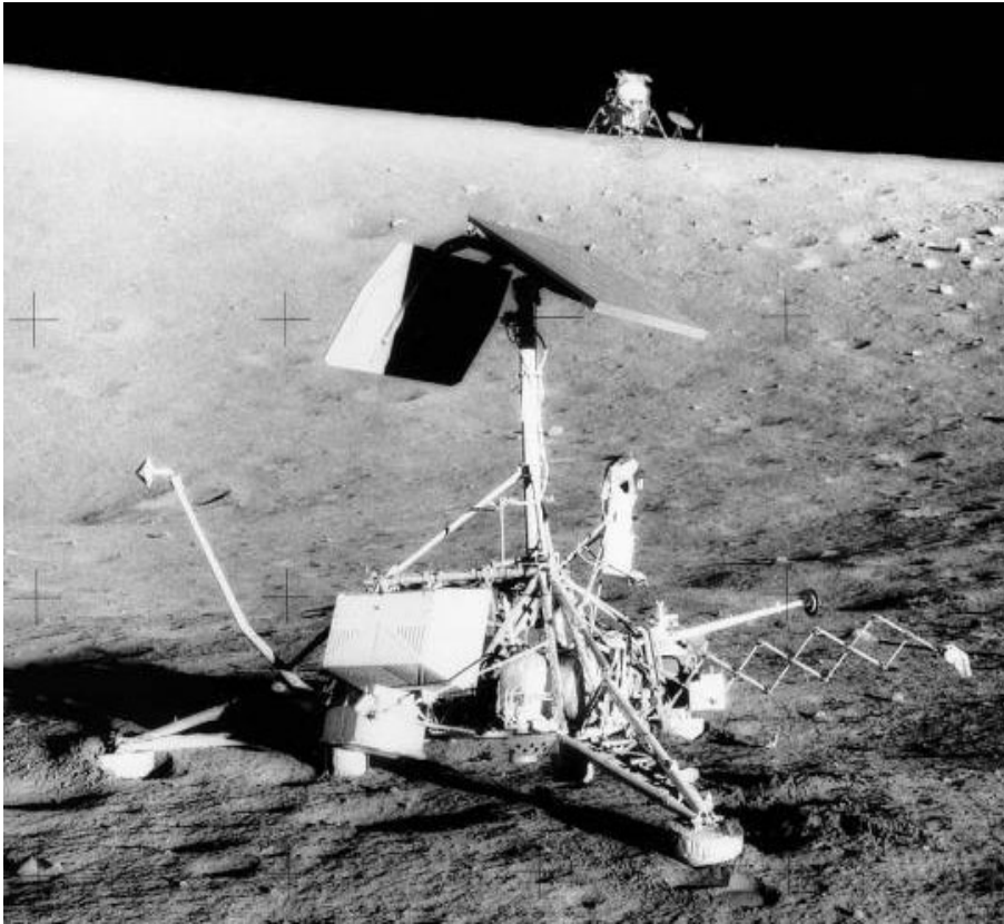
Figure 1. Surveyor 3 in 1969 after 31 months on the Moon. Apollo 12 lunar module in background.
