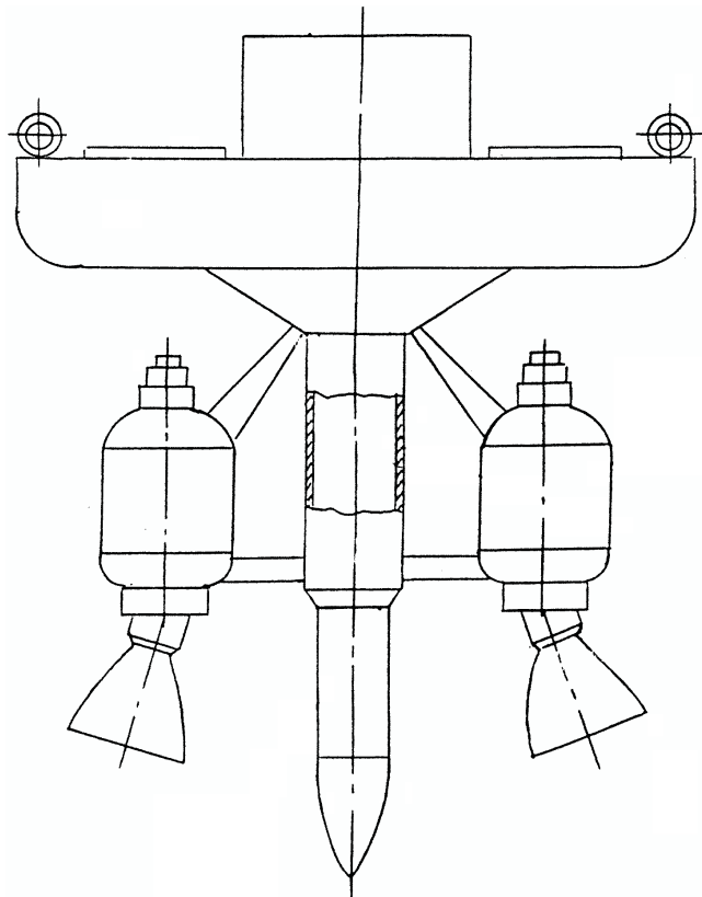
Figure 2. Design of the 'Luna-Glob' penetrator-lander.
