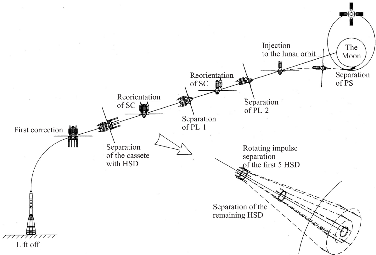
Figure 3. Schematic diagram of the mission profile of the 'Luna-Glob' project.
