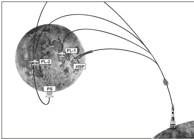
Figure 1. Lunar landing sites proposed in the Luna-Glob project. HSP – high-speed penetrators of the small aperture seismic array ( 18^{\circ}\text{S}, 38^{\circ}\text{N} ); PL-1 and PL-2 – penetrator-landers at 0.7^{\circ}\text{N}, 23.5^{\circ}\text{E} and 3^{\circ}\text{N}, 23.4^{\circ}\text{W} ; PS – Polar Station ( 88^{\circ}\text{S} ).
