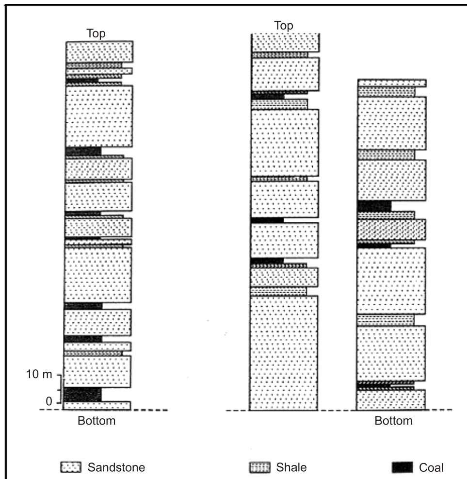
Figure 2. Subsurface Barakar stratigraphy of Bellampalli coalfield reproduced from borehole logs.
