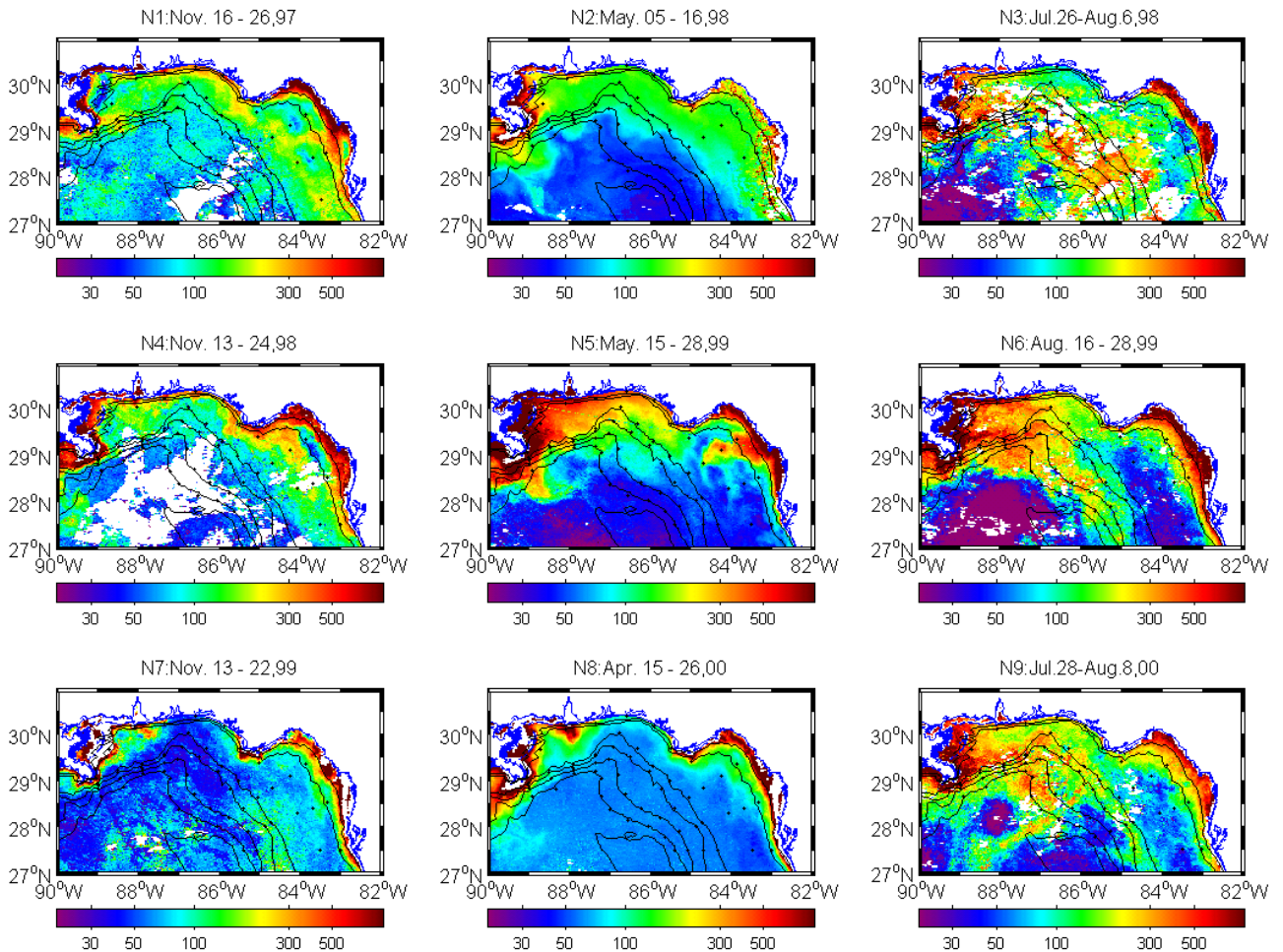
Figure 4. Estimated POC concentration ( \text{mg}/\text{m}^3 ) in the Northeastern Gulf of Mexico. Each map is compiled using PCA equation (5). POC estimates are well correlated with in situ data at both low and high POC concentrations.
