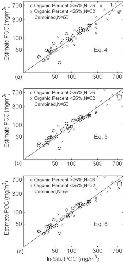
Figure 3. Comparisons between in situ POC and estimated POC using three different algorithms based on multiple linear regression and weighted PCA vectors. Data are delineated by percent organic carbon > 25% and < 25%. The lines are 1:1 slopes. All correlation statistics are in table 1.
