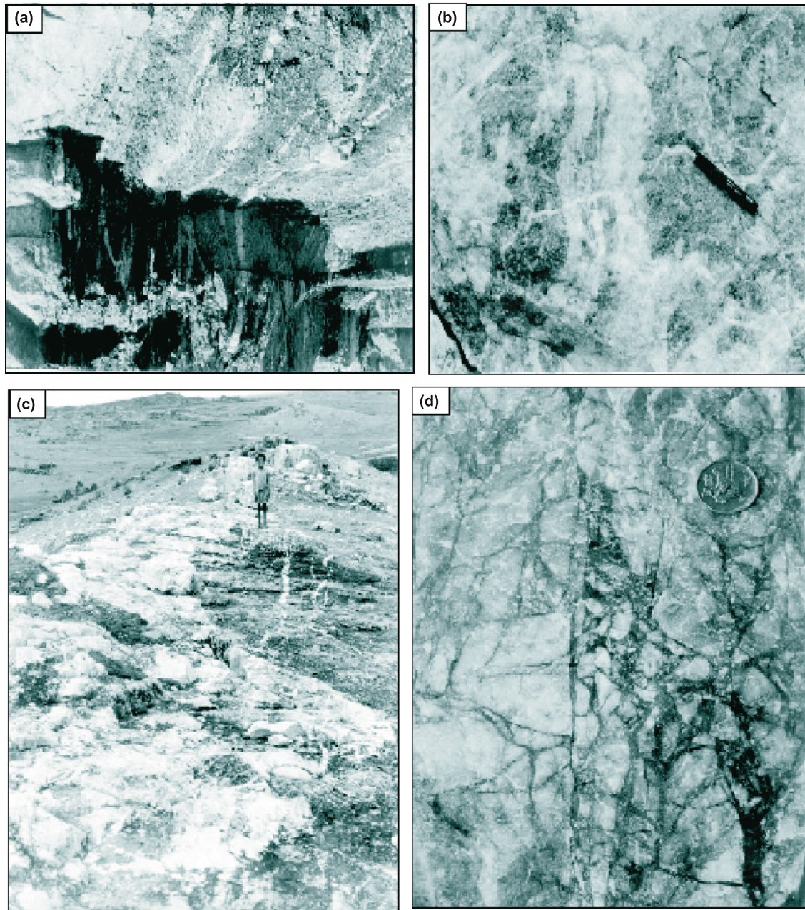
Figure 3. Field photographs. (a) Late generation thin quartz veins cut across the main vein suggesting multiple silica-rich solution activity in time and space in parts of Bundelkhand Craton. (b) Large granitoid clasts within giant quartz vein. Late generation thin quartz veins cut across the giant quartz vein as well as the granitoid clasts. (c) Giant quartz vein intruding the host coarse-grained pink granitoid ( \sim 2.5 Ga) with wavy contact. Some thin offshoot veins of quartz are present. (d) Breccia texture in giant quartz vein resulting from brittle deformation. Angular fragments of quartz are set in a fine-grained siliceous matrix.
