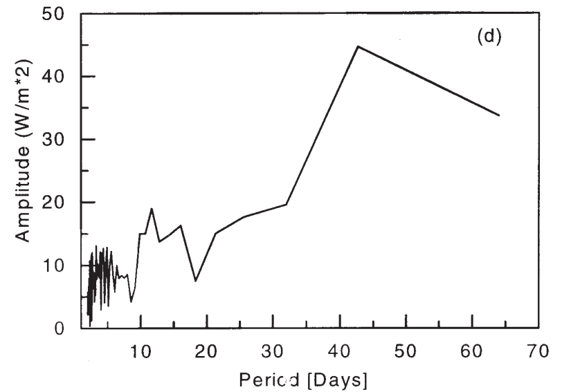
Figure 2(a-d). The power spectra for wind, SST, surface specific humidity and LHF over the Indian Ocean during 1999.
