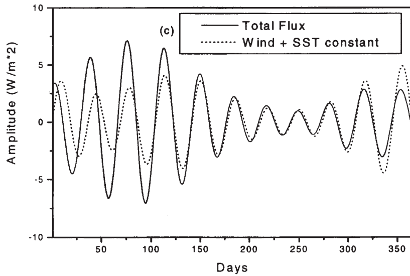
Figure 5(a-d). Same as figure 4(a-d) but for the Pacific Ocean.
