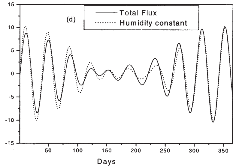
Figure 6(a-d). Same as figure 4(a-d) but for the Atlantic Ocean.
