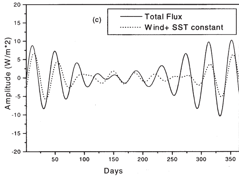
Figure 6(a-d). Same as figure 4(a-d) but for the Atlantic Ocean.
