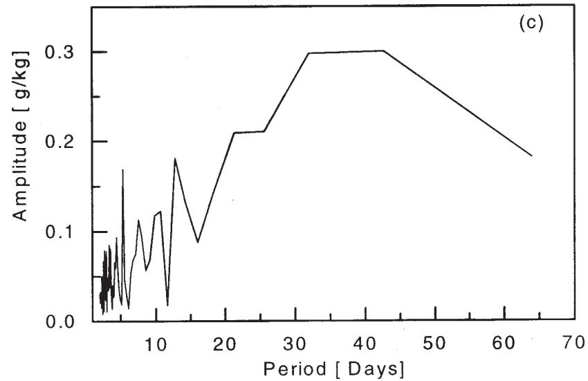
Figure 2(a-d). The power spectra for wind, SST, surface specific humidity and LHF over the Indian Ocean during 1999.
