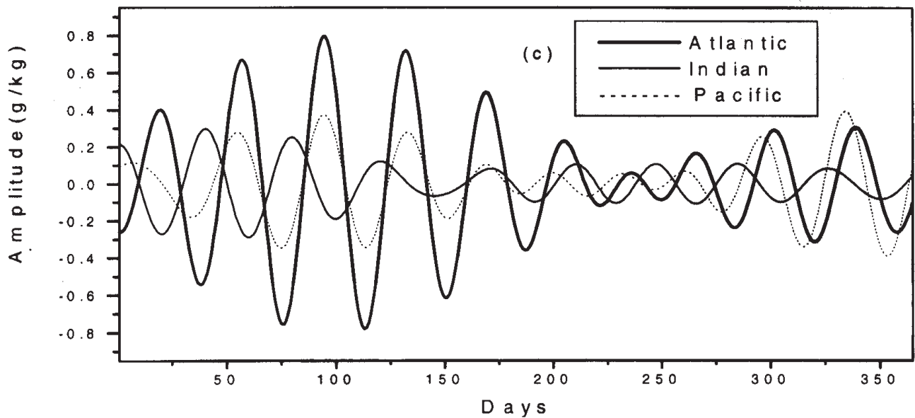
Figure 3(c). Same as figure 3(a) but for surface specific humidity.
