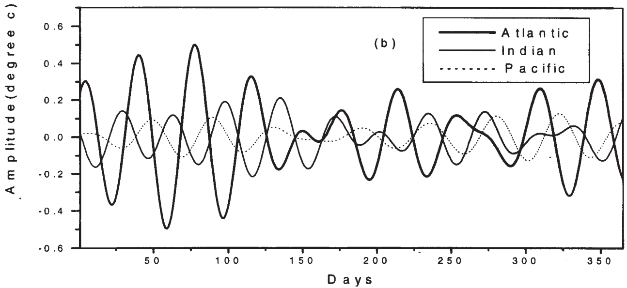
Figure 3(b). Same as figure 3(a) but for SST.
