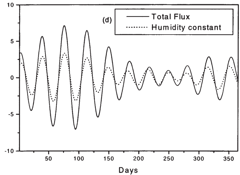
Figure 5(a-d). Same as figure 4(a-d) but for the Pacific Ocean.
