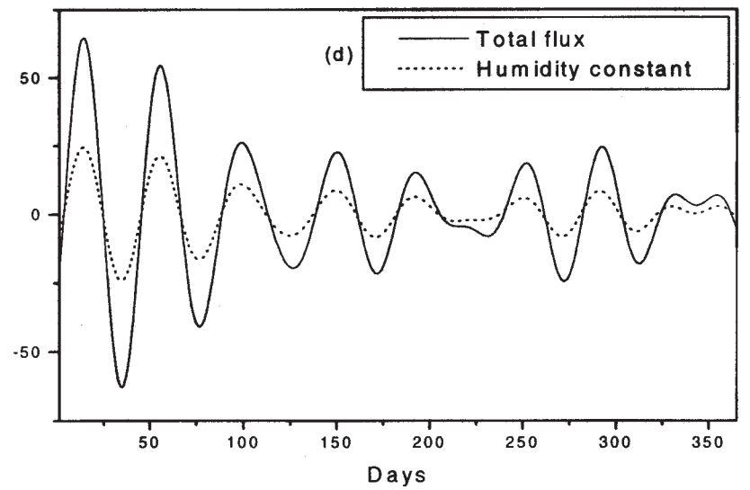
Figure 4(a-d). The impact on LHF Oscillation (30-50) by suppressing the oscillation in different variables over the Indian Ocean during 1999.
