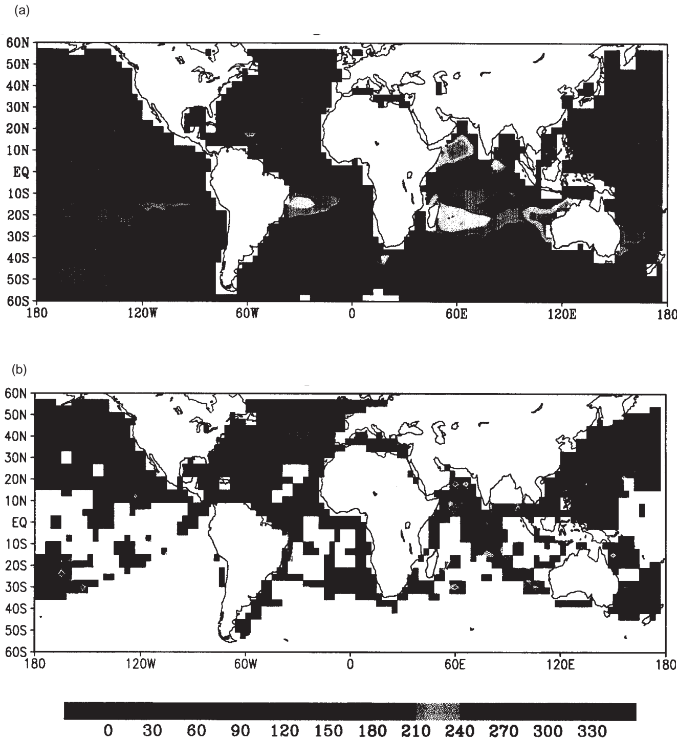
Figure 1. (a) The monthly mean LHF from NCEP for July 1999. (b) The monthly mean LHF from COADS for July 1999.
