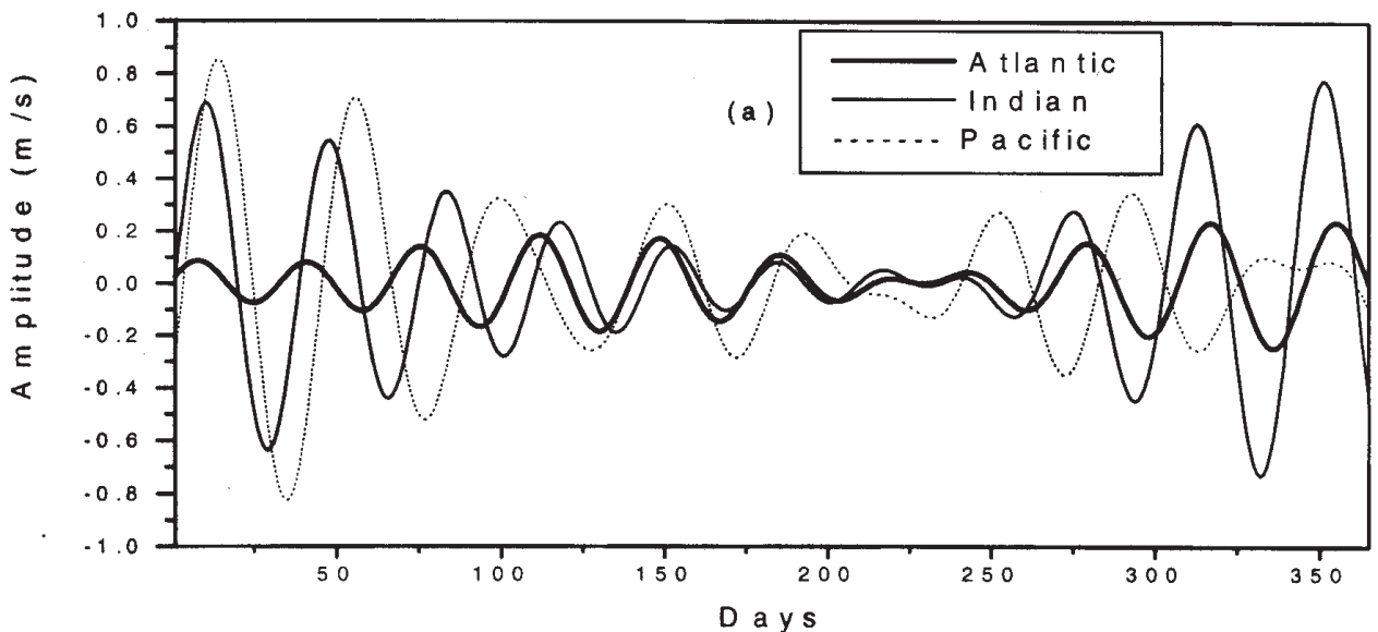
Figure 3(a). The time-filtered (30–50) series of wind over the three oceans during 1999.
