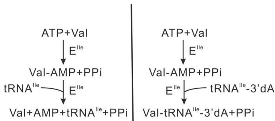
Figure 5. Valine is activated by Ile-tRNA synthetase but it is not transferred to tRNA Ile . In the absence of 3'-OH this erroneous aminoacylation occurs in high yield (van der Haar and Cramer 1975).
