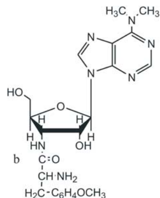
Figure 6. Structure of puromycin a nonisomerisable analogue of aminoacyl-tRNA.
