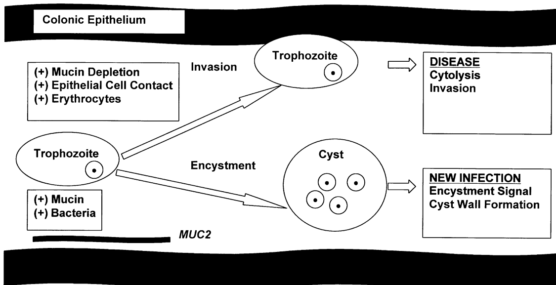
Figure 1. The life cycle of E. histolytica is carried out by its two forms encystation and invasive trophozoites. Local environmental cues signal via the Gal/GalNAc lectin and trigger encystation or invasion. Encystation may require bacterial flora and mucin binding. This form allows the cyst to leave the host and spread the infection to new individuals. The trophozoites cause tissue damage by use of the lectin to adhere and kill host cells. This figure is based on material accepted for publication in the Annual Review of Microbiology , volume 56, 2002 by Annual Reviews, www.AnnualReviews.org. Used with permission.
