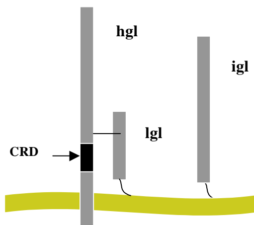
Figure 2. Gal/GalNAc adherence lectin of E. histolytica . The Gal/GalNAc lectin IS present of the surface amoeba and is comprised of three parts: hgl, lgl, and igl. Hgl and lgl are covalently linked and non-covalently associate with igl. Within hgl is the carbohydrate recognition domain (CRD). This region is believed to be responsible for the binding of hgl to host cells. Figure from Petri et al 2002 Annu. Rev. Microbiol. 56 39–64, printed with permission.
