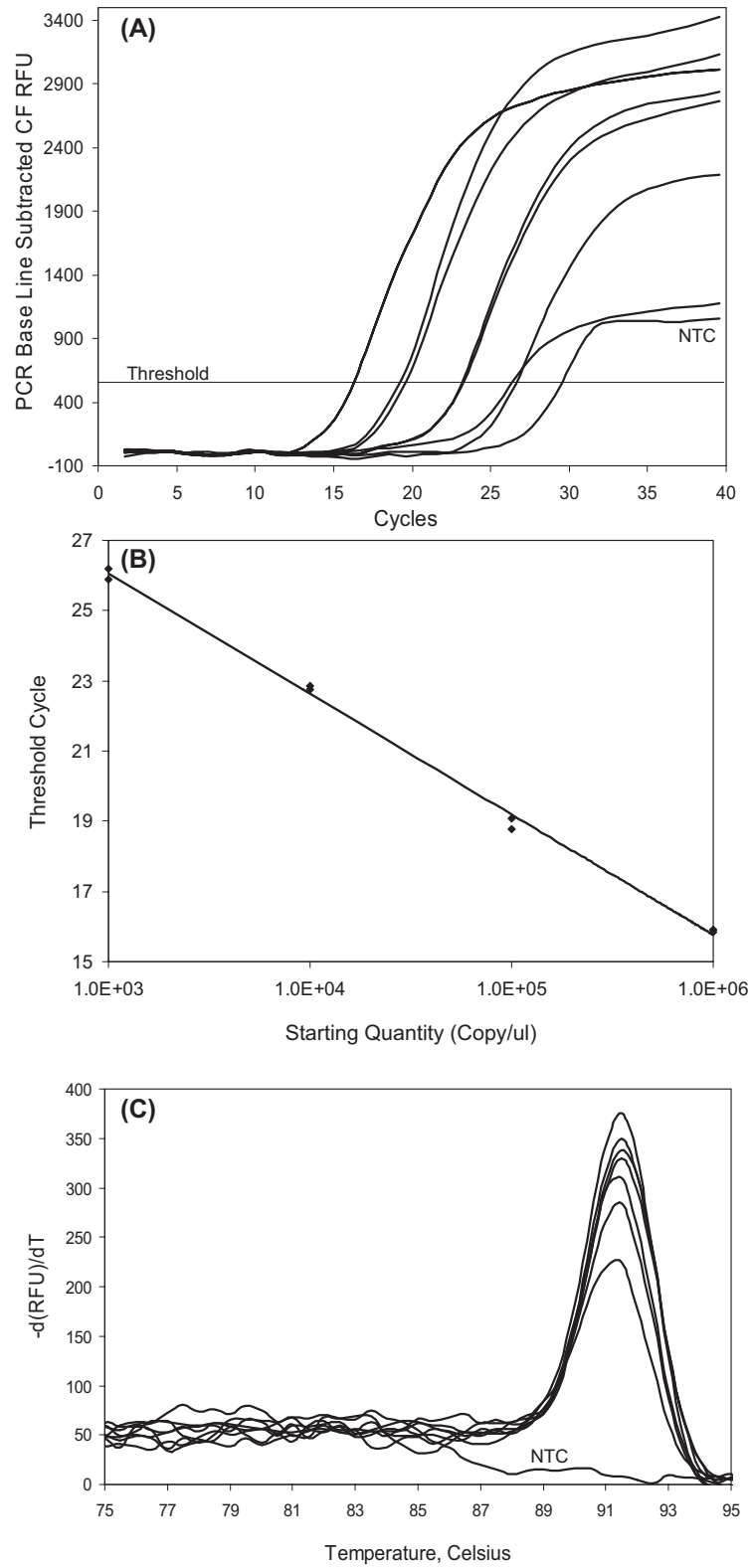
Figure 4. (A) Testing serial dilutions of template B ( 2.5 \times 10^3 - 2.5 \times 10^6 copies/ \mu l) using BOXTO with iCycler. (B) Standard curve indicating reaction efficiency = 95.6% and r^2 = 0.999 . (C) Inverted first derivative melting curve with a melting peak maximum at 91.5°C.
