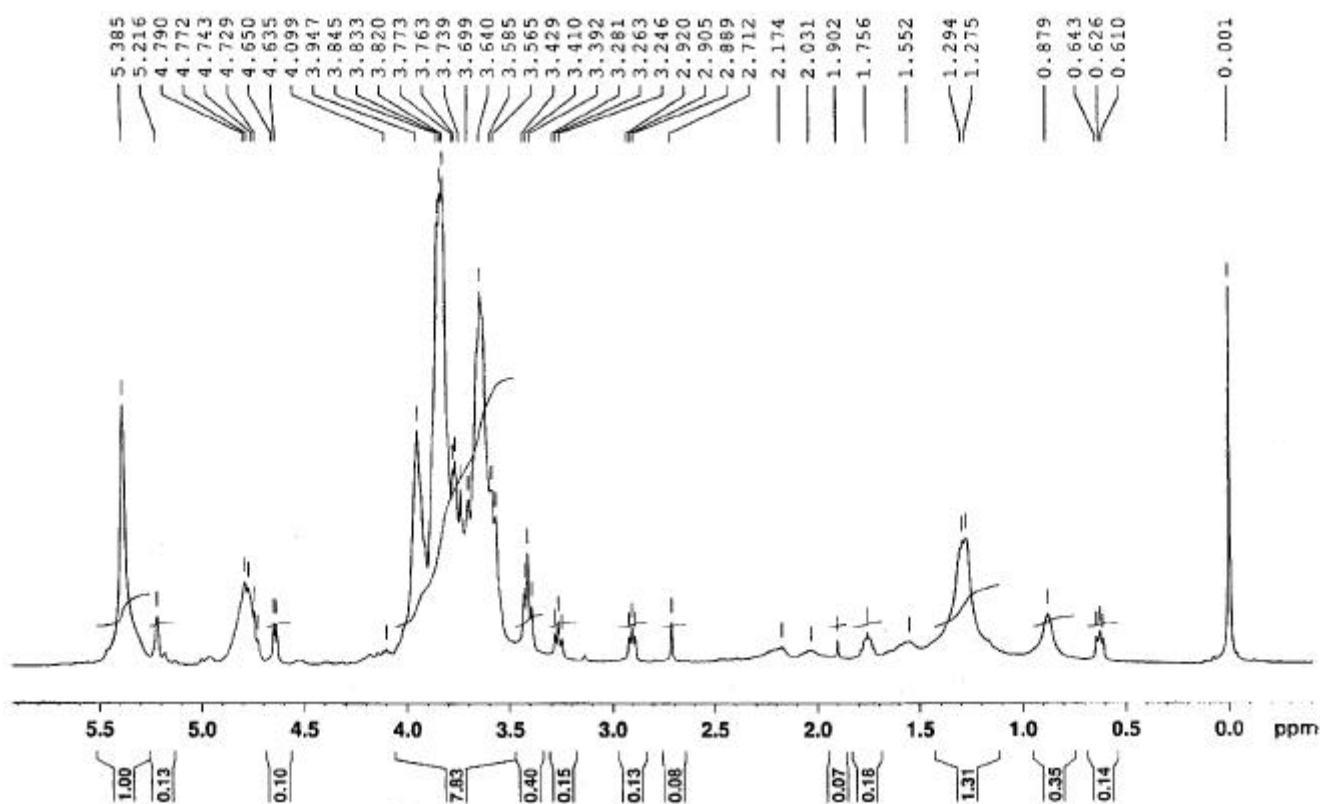
Figure 3. ^1\text{H} NMR spectrum of the antibiotic from S. albidoflavus PU 23. (The spectrum shows more than the expected peaks as it includes the peaks of the internal standard, DSS, and the solvent used.)
