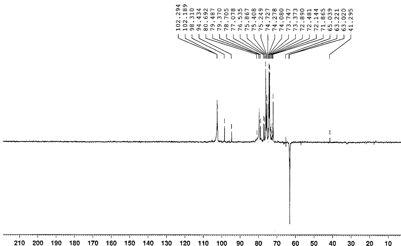
Figure 5. DEPT spectrum of the antibiotic from S. albidoflavus PU 23. (Internal standard-DSS.)
