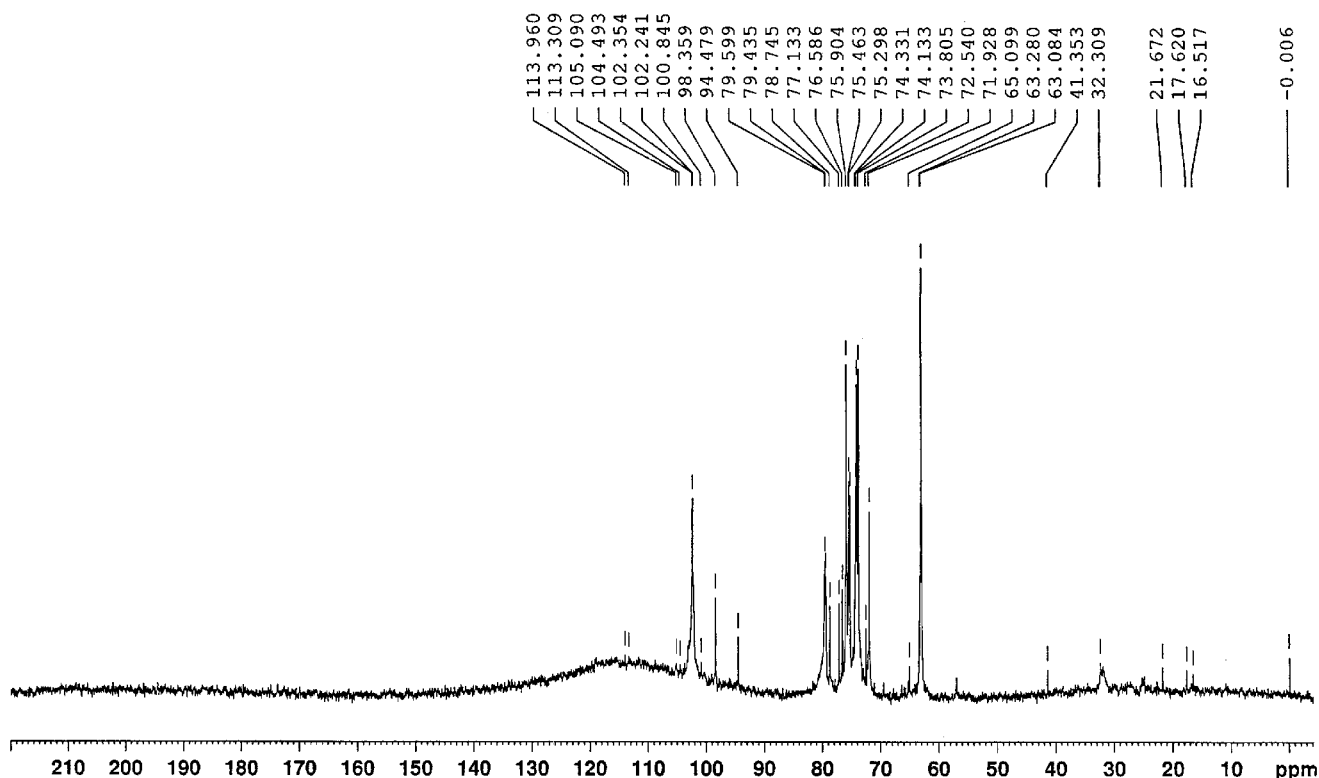
Figure 4. ^{13}\text{C} NMR spectrum of the antibiotic from S. albidoflavus PU 23. (The spectrum shows more than the expected peaks as it includes the peaks of the internal standard, DSS, and the solvent used.)
