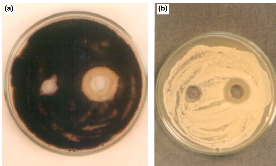
Figure 1. Antifungal activity exhibited by n-hexane extract of supernatant from S. albidoflavus PU 23 against (a) A. niger and (b) C. albicans (100 \mu\text{l} of the n-hexane extract was added in the wells. The well without the zone of inhibition is the control i.e. n-hexane).
