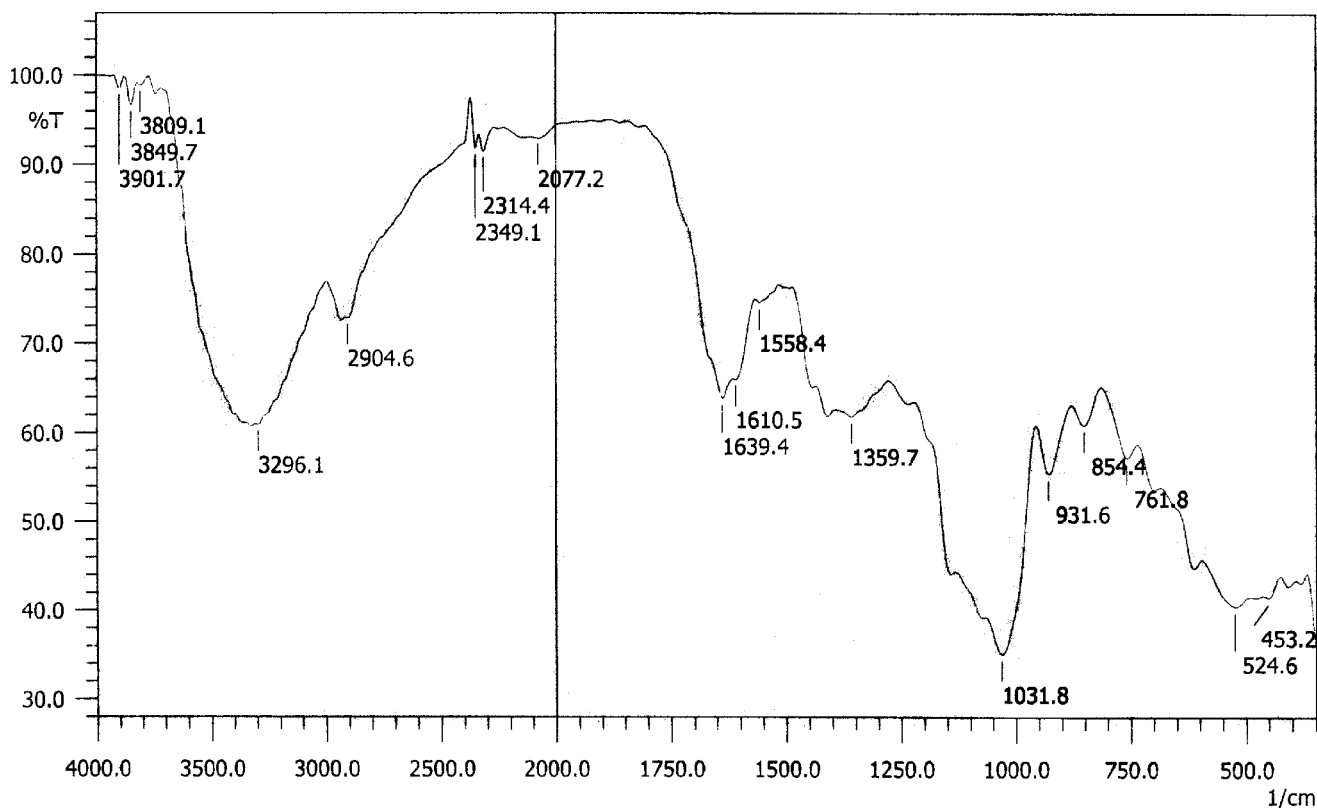
Figure 2. FTIR spectrum of the antibiotic from S. albidoflavus PU 23.
